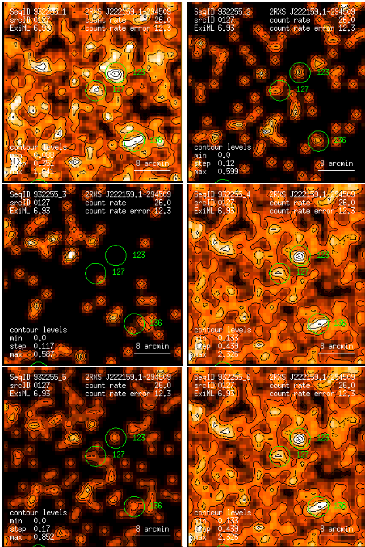
Figure 127: RASS 932255: detection 0127: band rate images, Gaussian filter: (1) PSPC channels 11 – 41, (2) 52 – 90, (3) 91 – 201, (4) 11 – 235, (5) 52 – 201, (6) 11 – 201. Broad band rates in counts/ks. Band rate contour levels in counts/ks/arcmin 2 .
