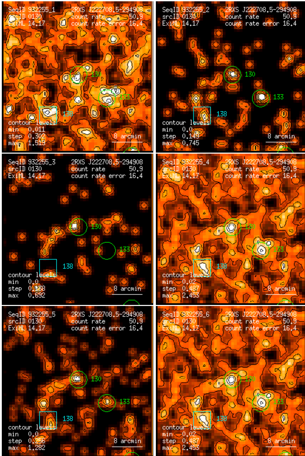
Figure 130: RASS 932255: detection 0130: band rate images, Gaussian filter: (1) PSPC channels 11 – 41, (2) 52 – 90, (3) 91 – 201, (4) 11 – 235, (5) 52 – 201, (6) 11 – 201. Broad band rates in counts/ks. Band rate contour levels in counts/ks/arcmin 2 .
