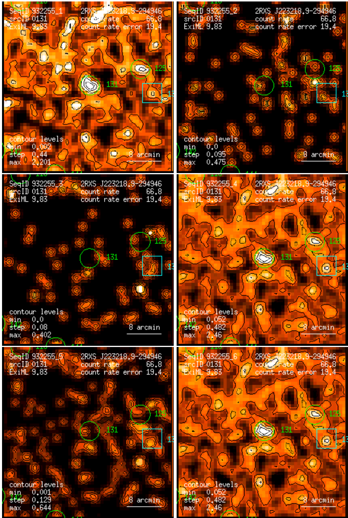
Figure 131: RASS 932255: detection 0131: band rate images, Gaussian filter: (1) PSPC channels 11 – 41, (2) 52 – 90, (3) 91 – 201, (4) 11 – 235, (5) 52 – 201, (6) 11 – 201. Broad band rates in counts/ks. Band rate contour levels in counts/ks/arcmin 2 .
