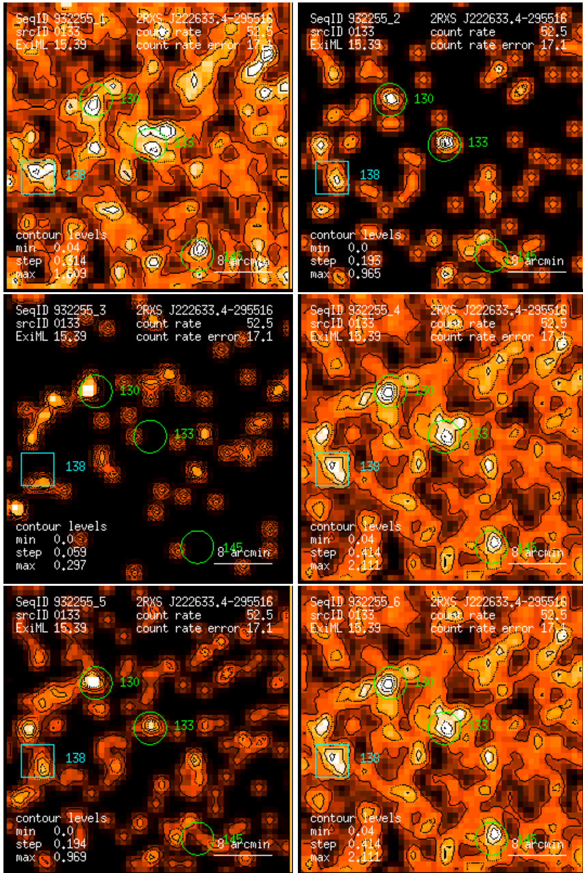
Figure 133: RASS 932255: detection 0133: band rate images, Gaussian filter: (1) PSPC channels 11 – 41, (2) 52 – 90, (3) 91 – 201, (4) 11 – 235, (5) 52 – 201, (6) 11 – 201. Broad band rates in counts/ks. Band rate contour levels in counts/ks/arcmin 2 .
