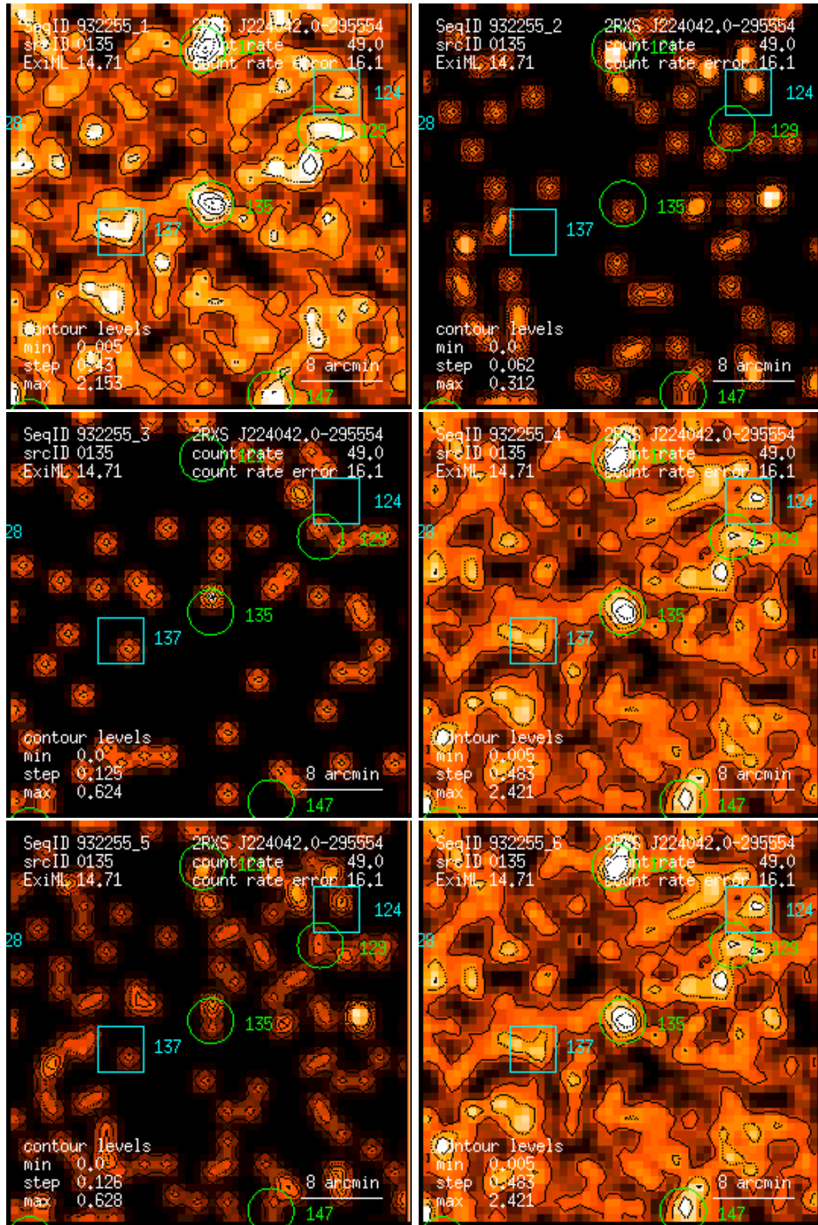
Figure 135: RASS 932255: detection 0135: band rate images, Gaussian filter: (1) PSPC channels 11 – 41, (2) 52 – 90, (3) 91 – 201, (4) 11 – 235, (5) 52 – 201, (6) 11 – 201. Broad band rates in counts/ks. Band rate contour levels in counts/ks/arcmin 2 .
