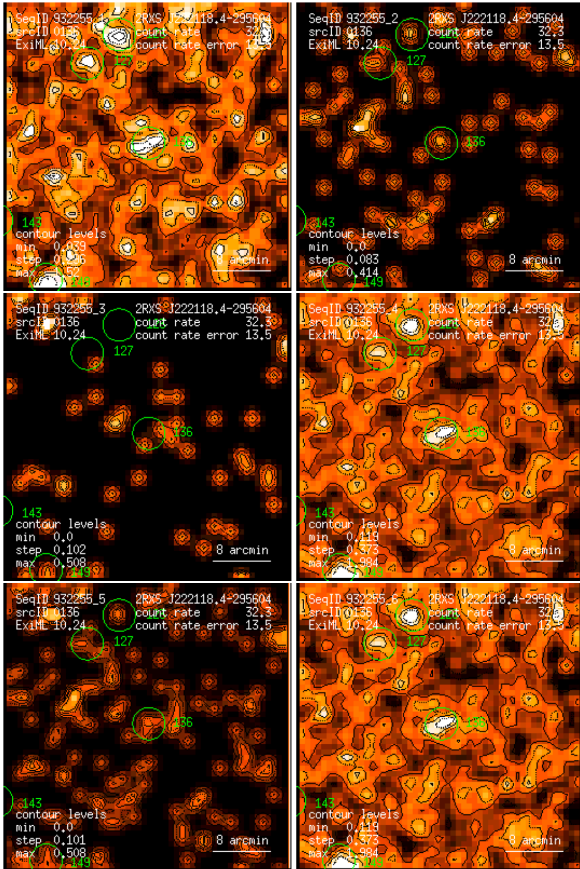
Figure 136: RASS 932255: detection 0136: band rate images, Gaussian filter: (1) PSPC channels 11 – 41, (2) 52 – 90, (3) 91 – 201, (4) 11 – 235, (5) 52 – 201, (6) 11 – 201. Broad band rates in counts/ks. Band rate contour levels in counts/ks/arcmin 2 .
