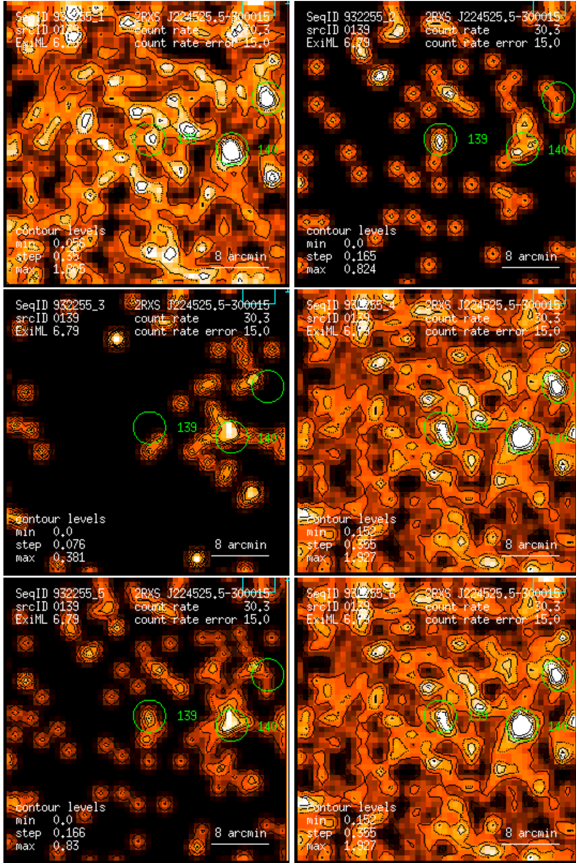
Figure 139: RASS 932255: detection 0139: band rate images, Gaussian filter: (1) PSPC channels 11 – 41, (2) 52 – 90, (3) 91 – 201, (4) 11 – 235, (5) 52 – 201, (6) 11 – 201. Broad band rates in counts/ks. Band rate contour levels in counts/ks/arcmin 2 .
