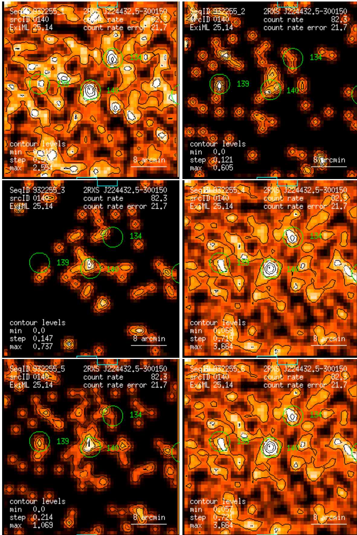
Figure 140: RASS 932255: detection 0140: band rate images, Gaussian filter: (1) PSPC channels 11 – 41, (2) 52 – 90, (3) 91 – 201, (4) 11 – 235, (5) 52 – 201, (6) 11 – 201. Broad band rates in counts/ks. Band rate contour levels in counts/ks/arcmin 2 .
