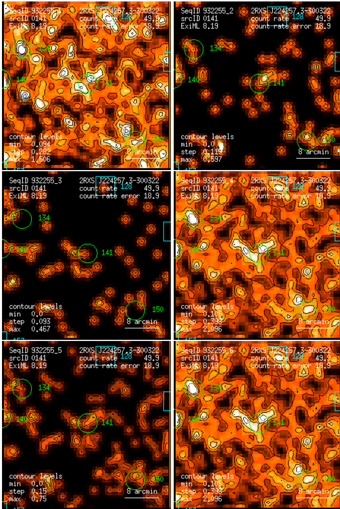
Figure 141: RASS 932255: detection 0141: band rate images, Gaussian filter: (1) PSPC channels 11 – 41, (2) 52 – 90, (3) 91 – 201, (4) 11 – 235, (5) 52 – 201, (6) 11 – 201. Broad band rates in counts/ks. Band rate contour levels in counts/ks/arcmin 2 .
