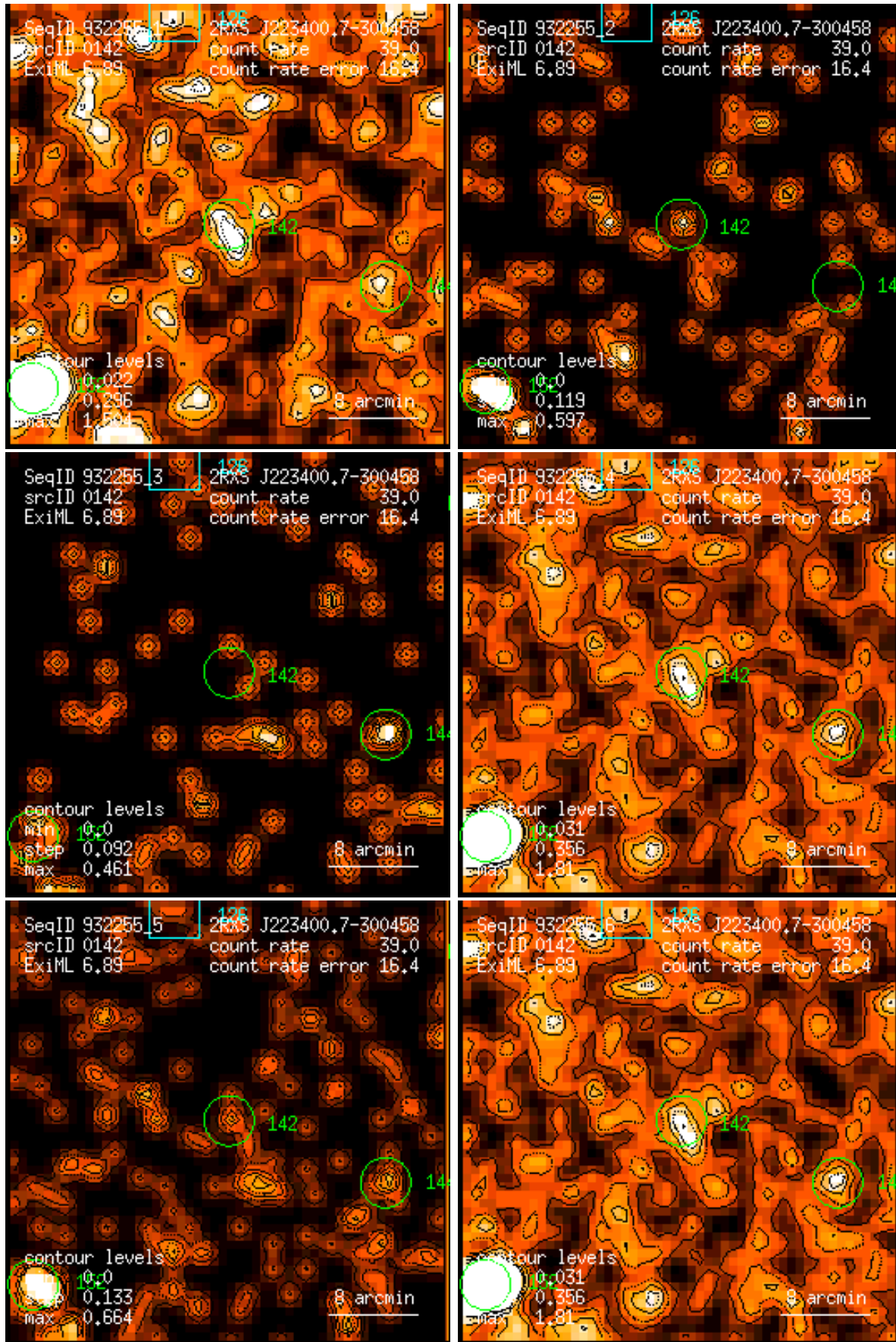
Figure 142: RASS 932255: detection 0142: band rate images, Gaussian filter: (1) PSPC channels 11 – 41, (2) 52 – 90, (3) 91 – 201, (4) 11 – 235, (5) 52 – 201, (6) 11 – 201. Broad band rates in counts/ks. Band rate contour levels in counts/ks/arcmin 2 .
