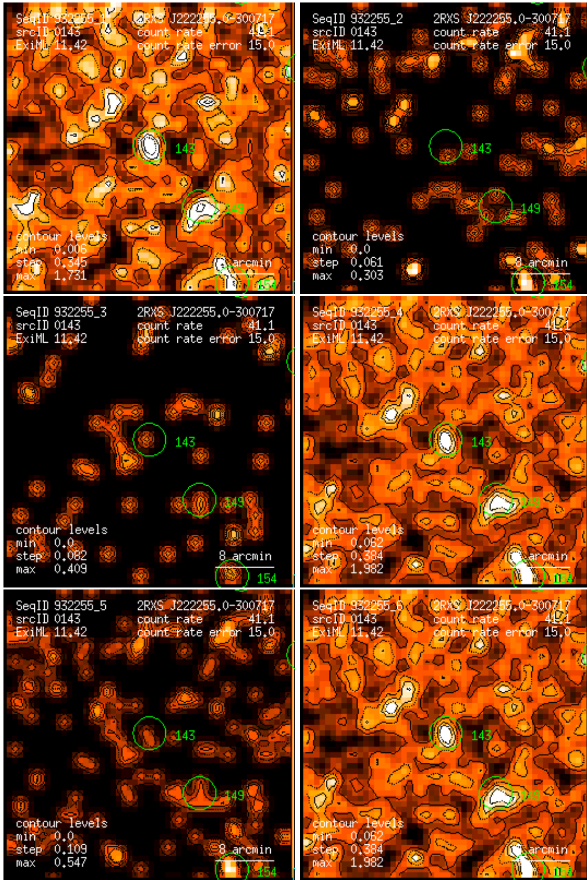
Figure 143: RASS 932255: detection 0143: band rate images, Gaussian filter: (1) PSPC channels 11 – 41, (2) 52 – 90, (3) 91 – 201, (4) 11 – 235, (5) 52 – 201, (6) 11 – 201. Broad band rates in counts/ks. Band rate contour levels in counts/ks/arcmin 2 .
