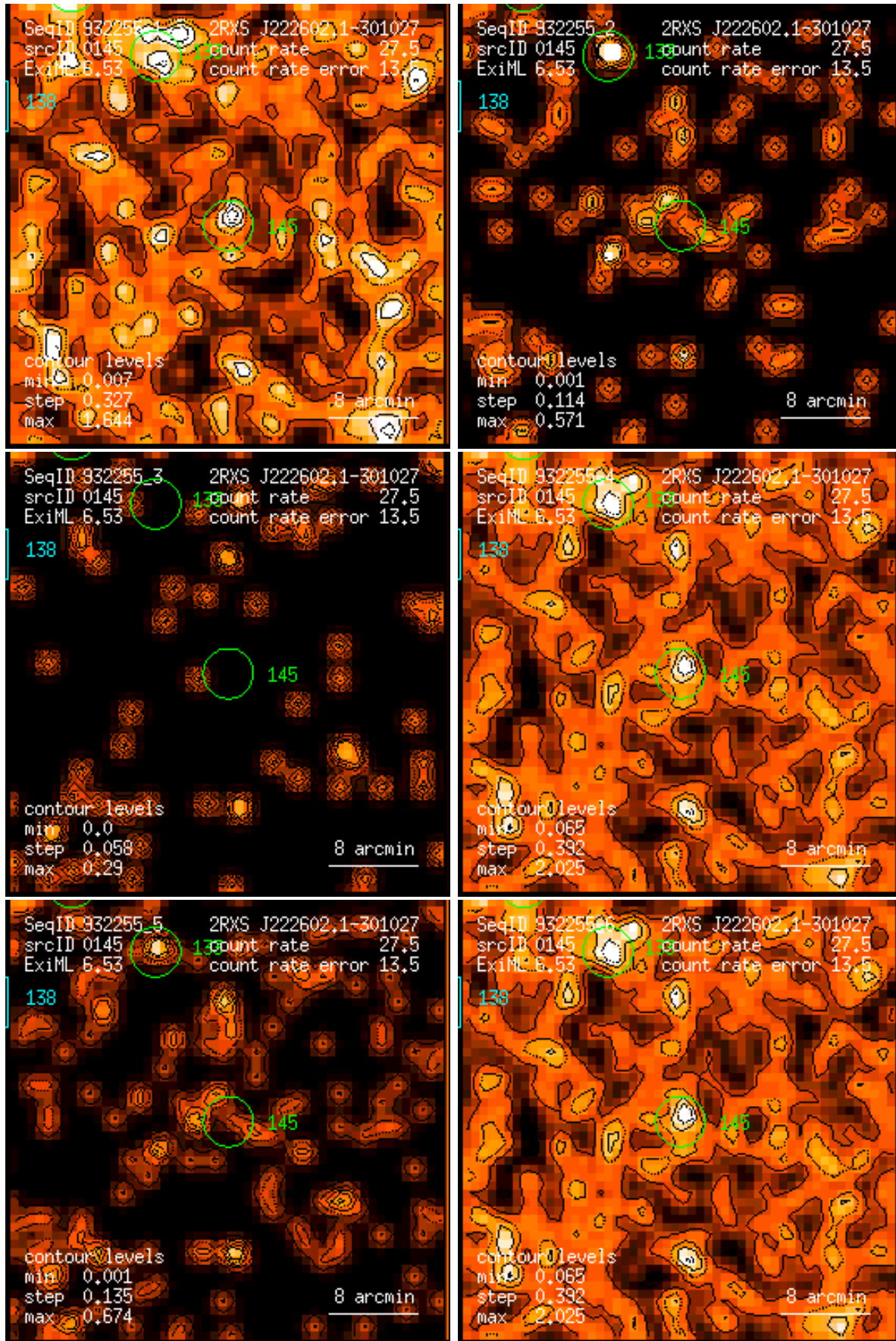
Figure 145: RASS 932255: detection 0145: band rate images, Gaussian filter: (1) PSPC channels 11 – 41, (2) 52 – 90, (3) 91 – 201, (4) 11 – 235, (5) 52 – 201, (6) 11 – 201. Broad band rates in counts/ks. Band rate contour levels in counts/ks/arcmin 2 .
