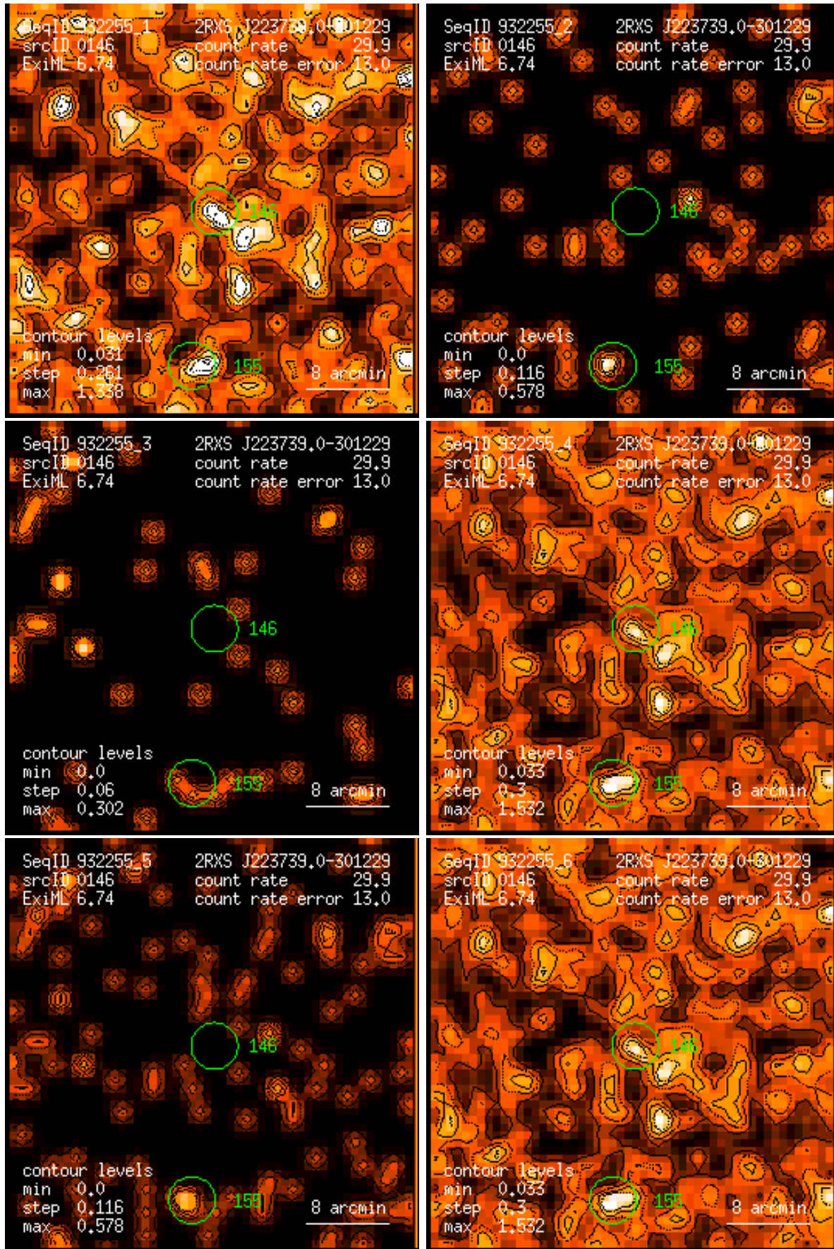
Figure 146: RASS 932255: detection 0146: band rate images, Gaussian filter: (1) PSPC channels 11 – 41, (2) 52 – 90, (3) 91 – 201, (4) 11 – 235, (5) 52 – 201, (6) 11 – 201. Broad band rates in counts/ks. Band rate contour levels in counts/ks/arcmin 2 .
