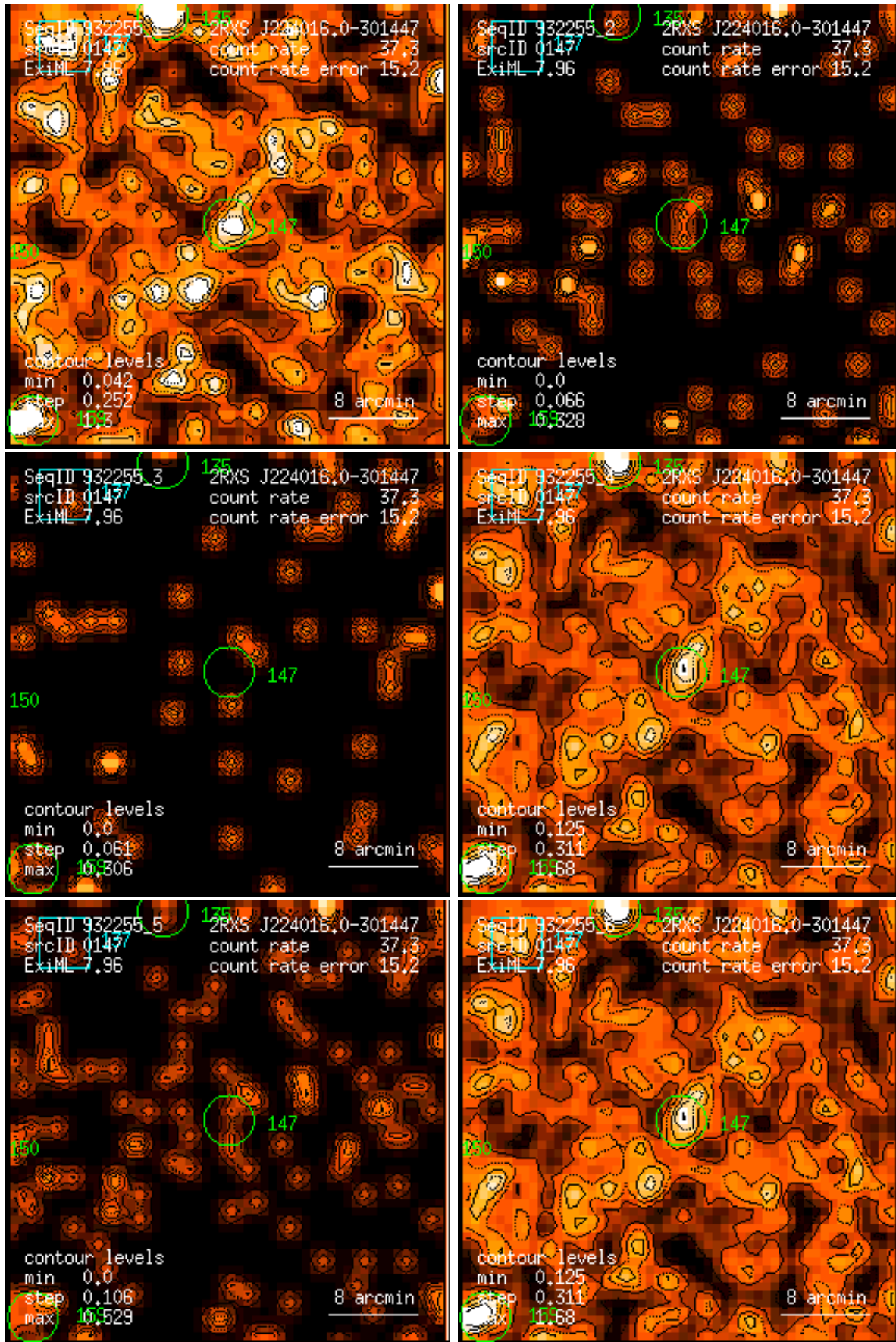
Figure 147: RASS 932255: detection 0147: band rate images, Gaussian filter: (1) PSPC channels 11 – 41, (2) 52 – 90, (3) 91 – 201, (4) 11 – 235, (5) 52 – 201, (6) 11 – 201. Broad band rates in counts/ks. Band rate contour levels in counts/ks/arcmin 2 .
