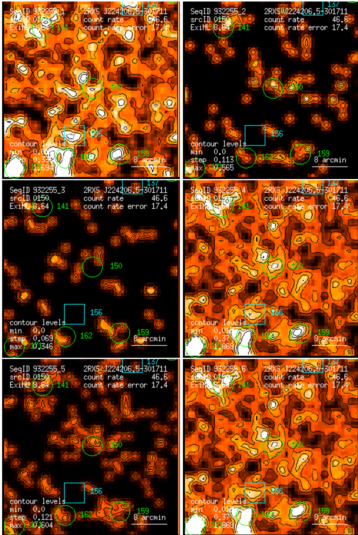
Figure 150: RASS 932255: detection 0150: band rate images, Gaussian filter: (1) PSPC channels 11 – 41, (2) 52 – 90, (3) 91 – 201, (4) 11 – 235, (5) 52 – 201, (6) 11 – 201. Broad band rates in counts/ks. Band rate contour levels in counts/ks/arcmin 2 .
