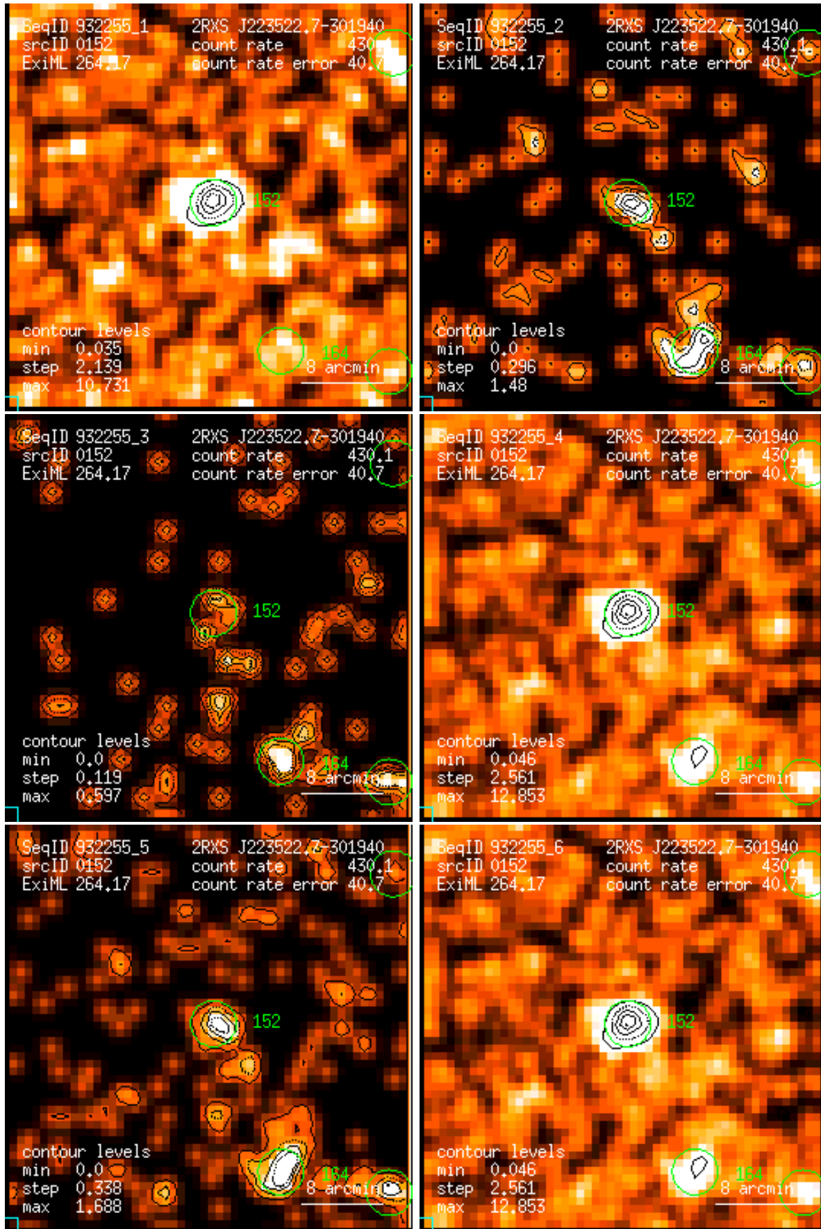
Figure 152: RASS 932255: detection 0152: band rate images, Gaussian filter: (1) PSPC channels 11 – 41, (2) 52 – 90, (3) 91 – 201, (4) 11 – 235, (5) 52 – 201, (6) 11 – 201. Broad band rates in counts/ks. Band rate contour levels in counts/ks/arcmin 2 .
