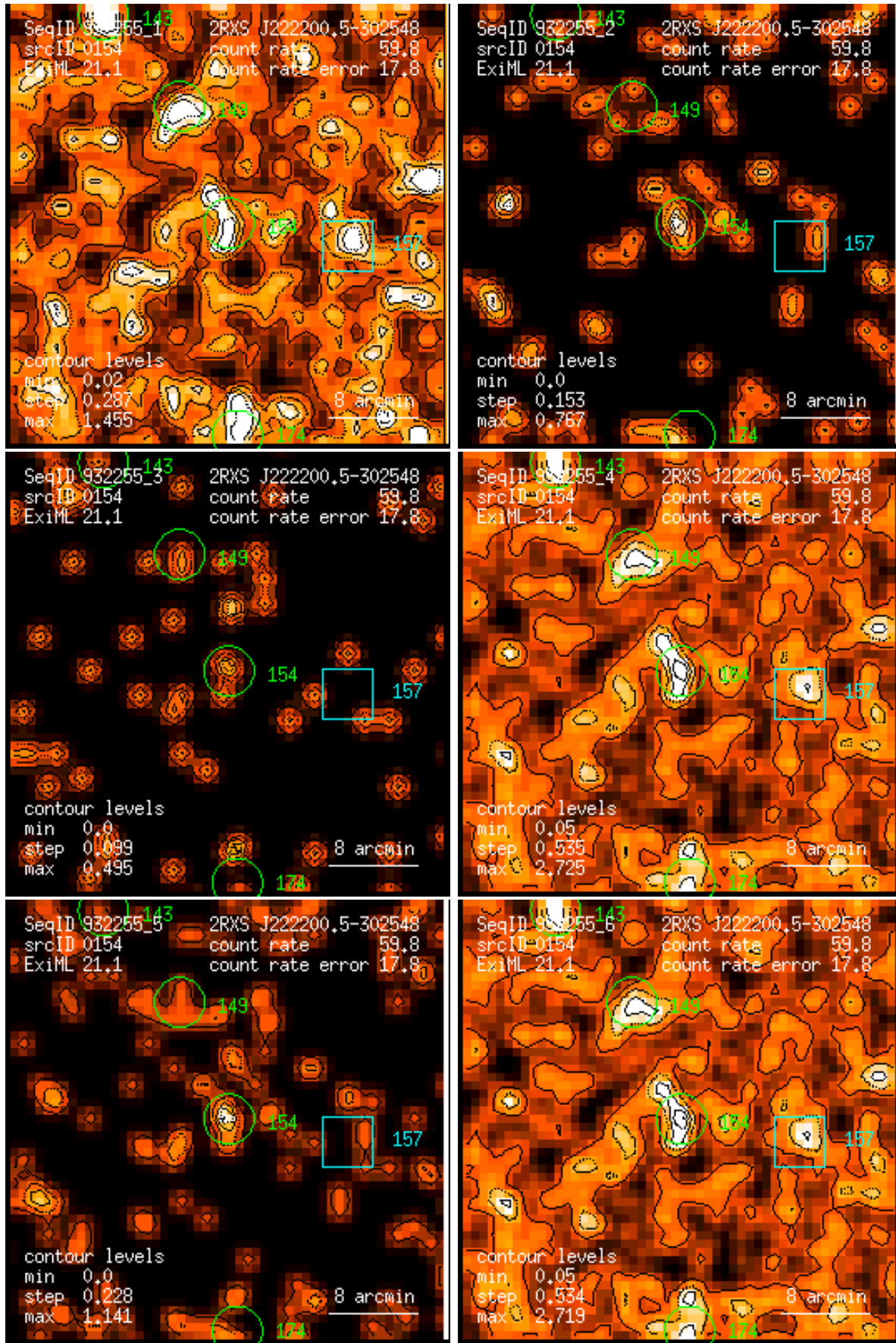
Figure 154: RASS 932255: detection 0154: band rate images, Gaussian filter: (1) PSPC channels 11 – 41, (2) 52 – 90, (3) 91 – 201, (4) 11 – 235, (5) 52 – 201, (6) 11 – 201. Broad band rates in counts/ks. Band rate contour levels in counts/ks/arcmin 2 .
