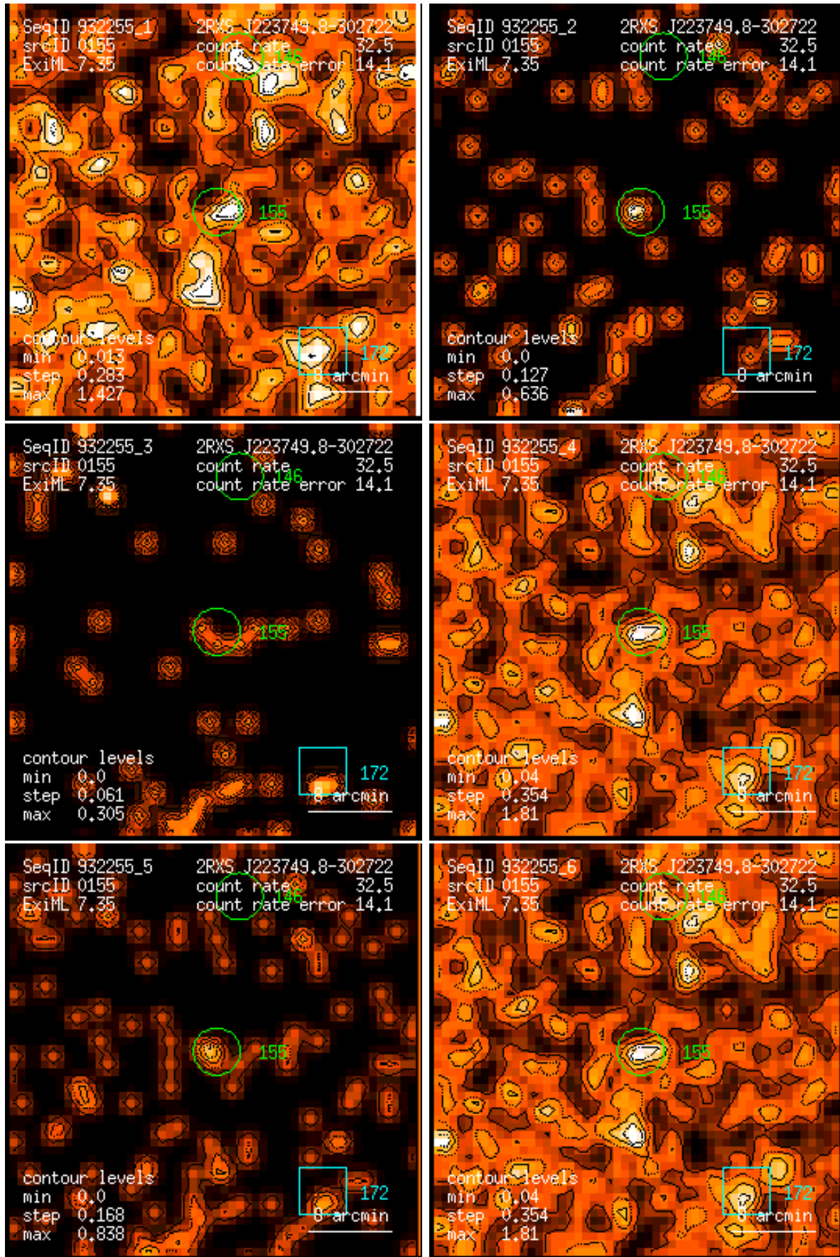
Figure 155: RASS 932255: detection 0155: band rate images, Gaussian filter: (1) PSPC channels 11 – 41, (2) 52 – 90, (3) 91 – 201, (4) 11 – 235, (5) 52 – 201, (6) 11 – 201. Broad band rates in counts/ks. Band rate contour levels in counts/ks/arcmin 2 .
