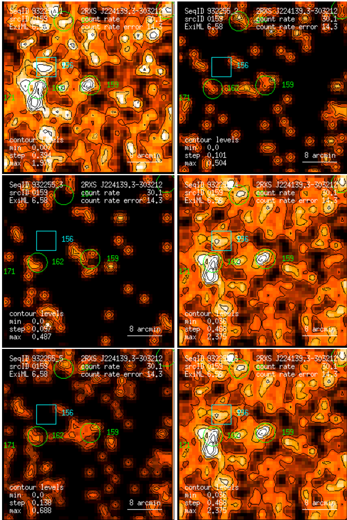
Figure 159: RASS 932255: detection 0159: band rate images, Gaussian filter: (1) PSPC channels 11 – 41, (2) 52 – 90, (3) 91 – 201, (4) 11 – 235, (5) 52 – 201, (6) 11 – 201. Broad band rates in counts/ks. Band rate contour levels in counts/ks/arcmin 2 .
