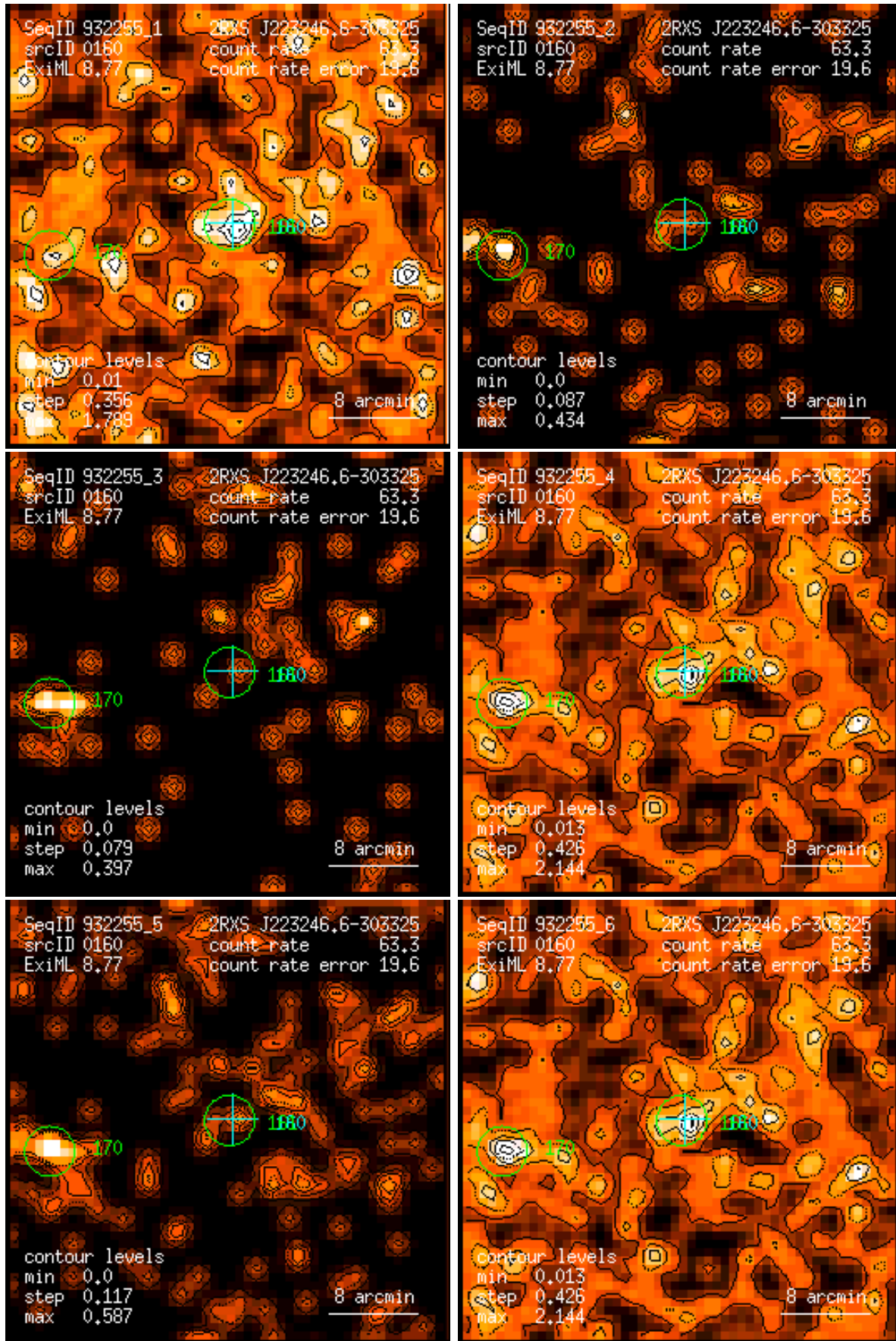
Figure 160: RASS 932255: detection 0160: band rate images, Gaussian filter: (1) PSPC channels 11 – 41, (2) 52 – 90, (3) 91 – 201, (4) 11 – 235, (5) 52 – 201, (6) 11 – 201. Broad band rates in counts/ks. Band rate contour levels in counts/ks/arcmin 2 .
