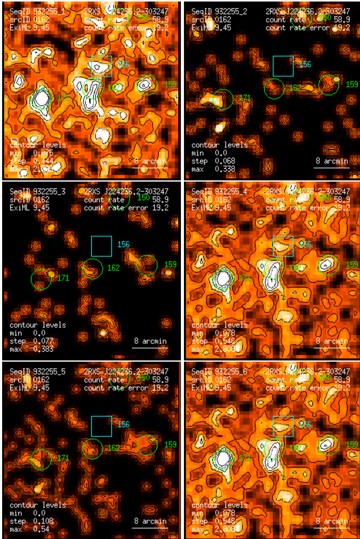
Figure 162: RASS 932255: detection 0162: band rate images, Gaussian filter: (1) PSPC channels 11 – 41, (2) 52 – 90, (3) 91 – 201, (4) 11 – 235, (5) 52 – 201, (6) 11 – 201. Broad band rates in counts/ks. Band rate contour levels in counts/ks/arcmin 2 .
