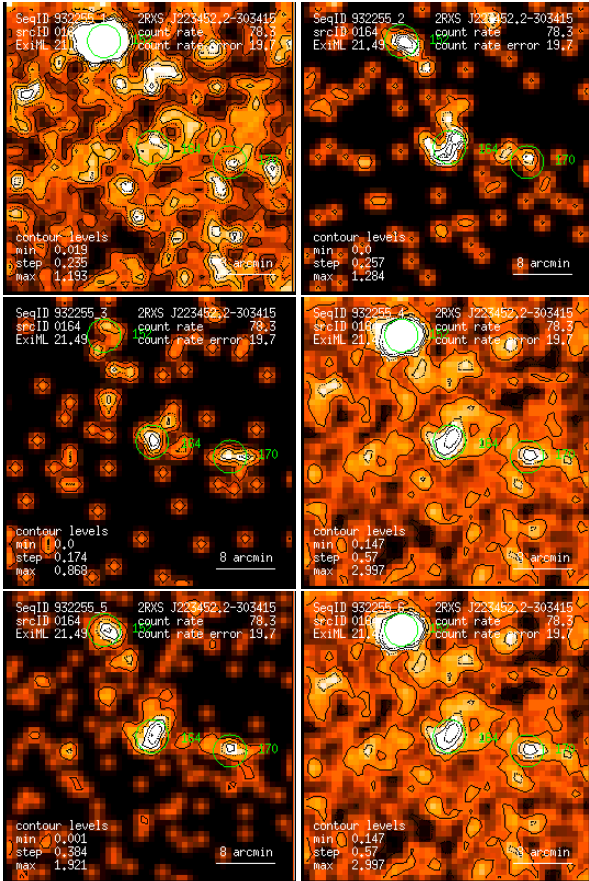
Figure 164: RASS 932255: detection 0164: band rate images, Gaussian filter: (1) PSPC channels 11 – 41, (2) 52 – 90, (3) 91 – 201, (4) 11 – 235, (5) 52 – 201, (6) 11 – 201. Broad band rates in counts/ks. Band rate contour levels in counts/ks/arcmin 2 .
