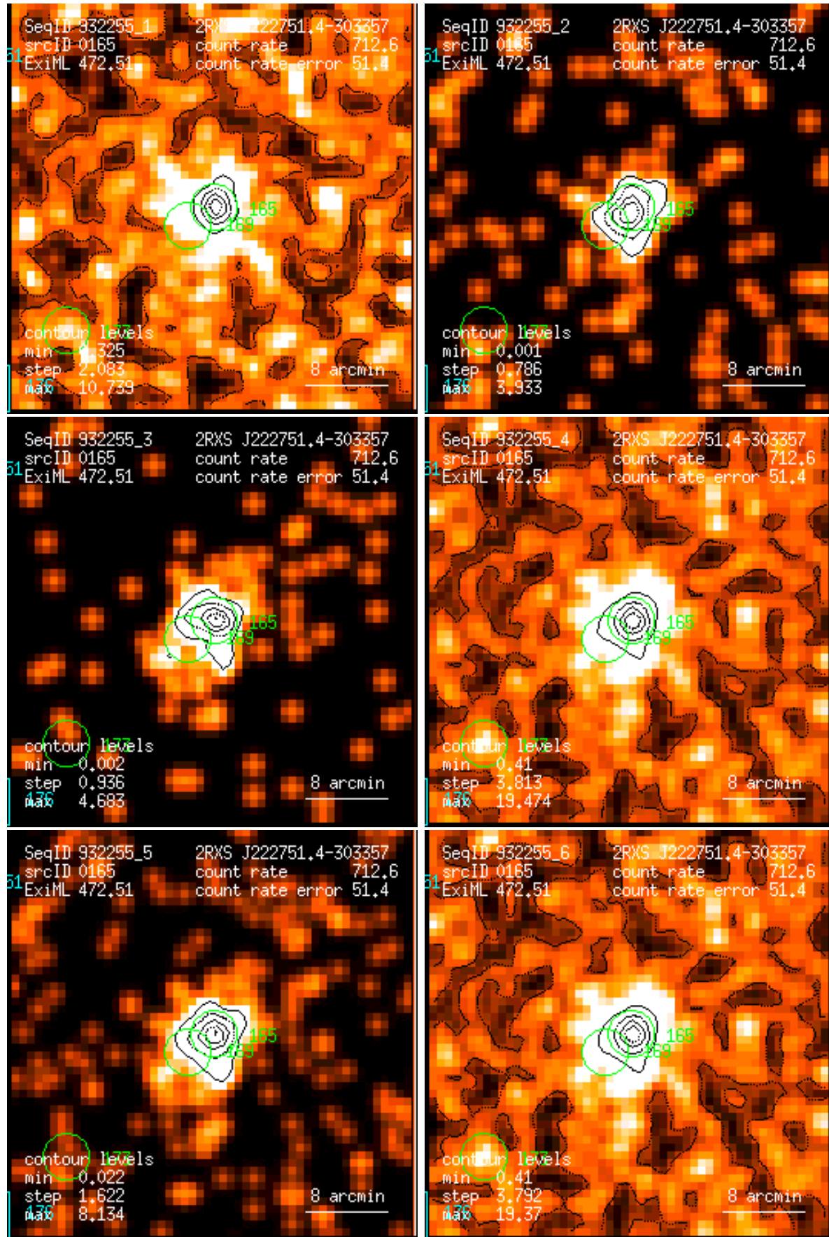
Figure 165: RASS 932255: detection 0165: band rate images, Gaussian filter: (1) PSPC channels 11 – 41, (2) 52 – 90, (3) 91 – 201, (4) 11 – 235, (5) 52 – 201, (6) 11 – 201. Broad band rates in counts/ks. Band rate contour levels in counts/ks/arcmin 2 .
