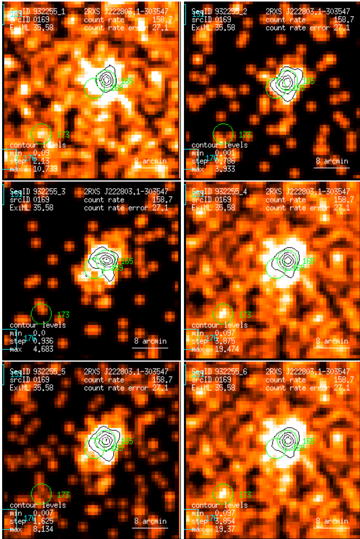
Figure 169: RASS 932255: detection 0169: band rate images, Gaussian filter: (1) PSPC channels 11 – 41, (2) 52 – 90, (3) 91 – 201, (4) 11 – 235, (5) 52 – 201, (6) 11 – 201. Broad band rates in counts/ks. Band rate contour levels in counts/ks/arcmin 2 .
