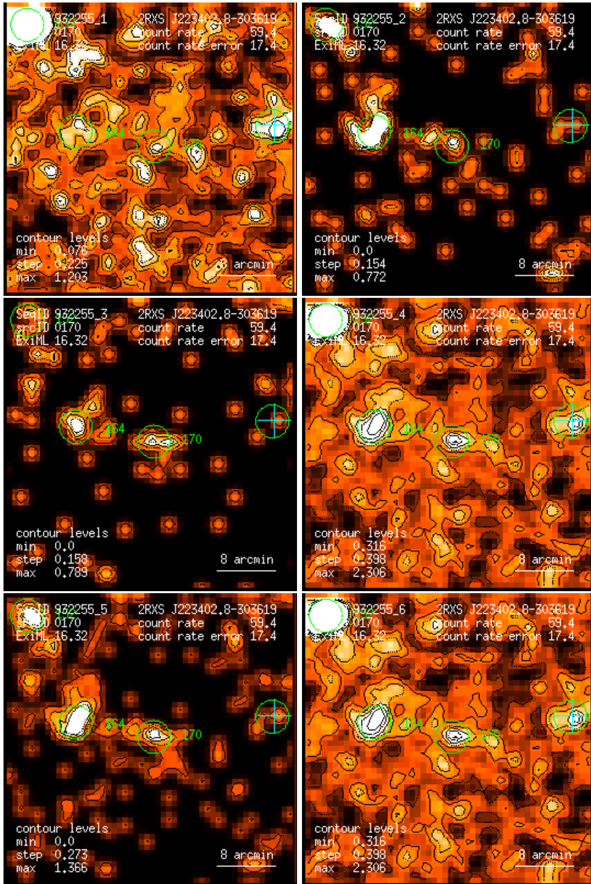
Figure 170: RASS 932255: detection 0170: band rate images, Gaussian filter: (1) PSPC channels 11 – 41, (2) 52 – 90, (3) 91 – 201, (4) 11 – 235, (5) 52 – 201, (6) 11 – 201. Broad band rates in counts/ks. Band rate contour levels in counts/ks/arcmin 2 .
