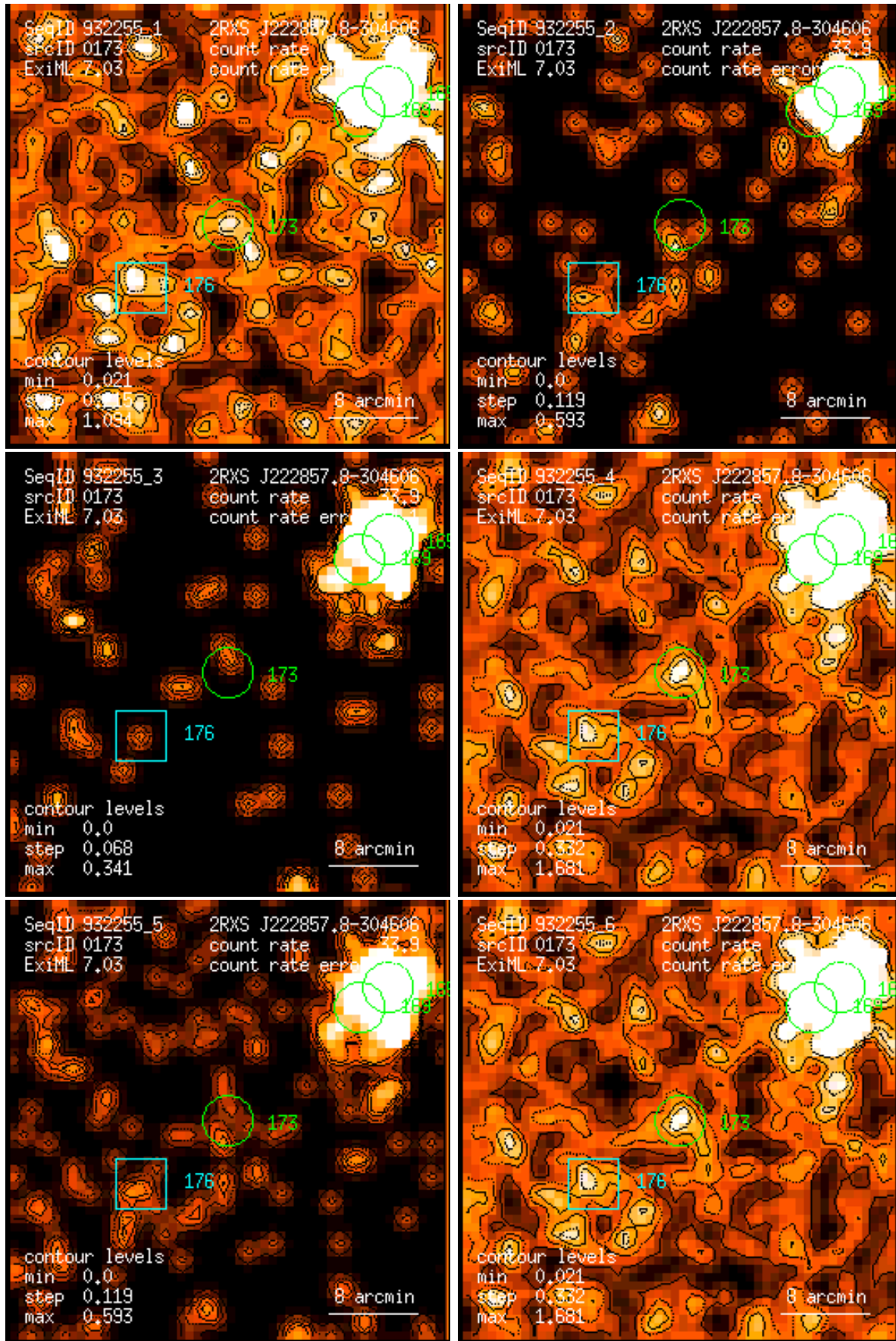
Figure 173: RASS 932255: detection 0173: band rate images, Gaussian filter: (1) PSPC channels 11 – 41, (2) 52 – 90, (3) 91 – 201, (4) 11 – 235, (5) 52 – 201, (6) 11 – 201. Broad band rates in counts/ks. Band rate contour levels in counts/ks/arcmin 2 .
