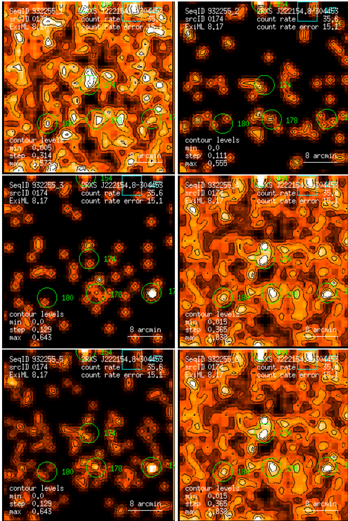
Figure 174: RASS 932255: detection 0174: band rate images, Gaussian filter: (1) PSPC channels 11 – 41, (2) 52 – 90, (3) 91 – 201, (4) 11 – 235, (5) 52 – 201, (6) 11 – 201. Broad band rates in counts/ks. Band rate contour levels in counts/ks/arcmin 2 .
