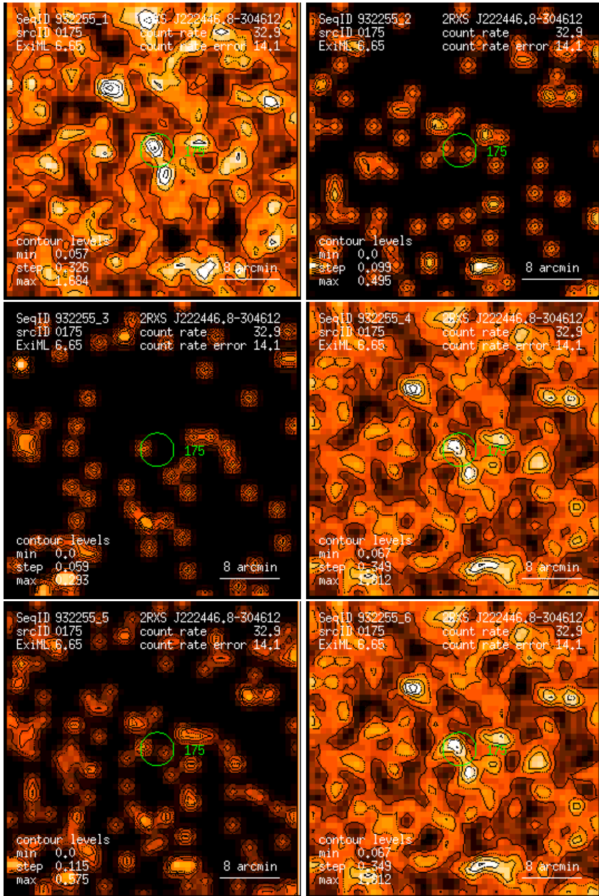
Figure 175: RASS 932255: detection 0175: band rate images, Gaussian filter: (1) PSPC channels 11 – 41, (2) 52 – 90, (3) 91 – 201, (4) 11 – 235, (5) 52 – 201, (6) 11 – 201. Broad band rates in counts/ks. Band rate contour levels in counts/ks/arcmin 2 .
