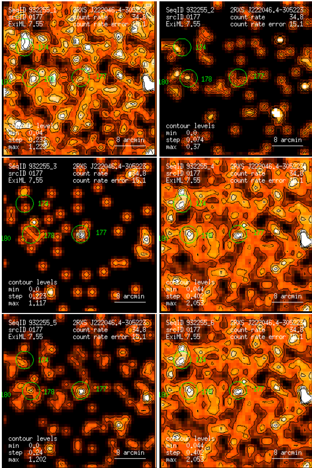
Figure 177: RASS 932255: detection 0177: band rate images, Gaussian filter: (1) PSPC channels 11 – 41, (2) 52 – 90, (3) 91 – 201, (4) 11 – 235, (5) 52 – 201, (6) 11 – 201. Broad band rates in counts/ks. Band rate contour levels in counts/ks/arcmin 2 .
