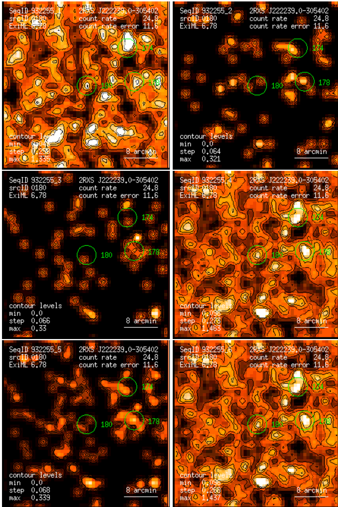
Figure 180: RASS 932255: detection 0180: band rate images, Gaussian filter: (1) PSPC channels 11 – 41, (2) 52 – 90, (3) 91 – 201, (4) 11 – 235, (5) 52 – 201, (6) 11 – 201. Broad band rates in counts/ks. Band rate contour levels in counts/ks/arcmin 2 .
