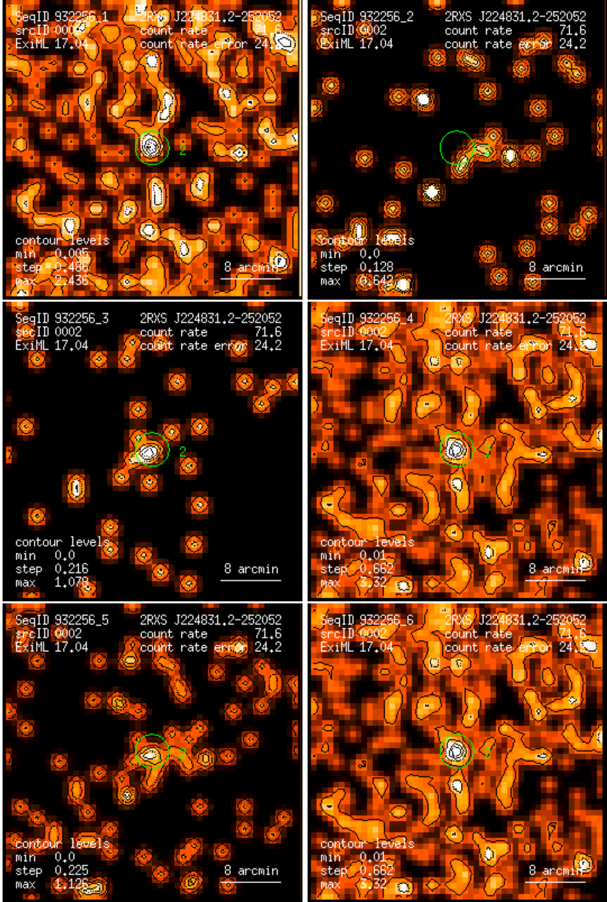
Figure 2: RASS 932256: detection 0002: band rate images, Gaussian filter: (1) PSPC channels 11 – 41, (2) 52 – 90, (3) 91 – 201, (4) 11 – 235, (5) 52 – 201, (6) 11 – 201. Broad band rates in counts/ks. Band rate contour levels in counts/ks/arcmin 2 .
