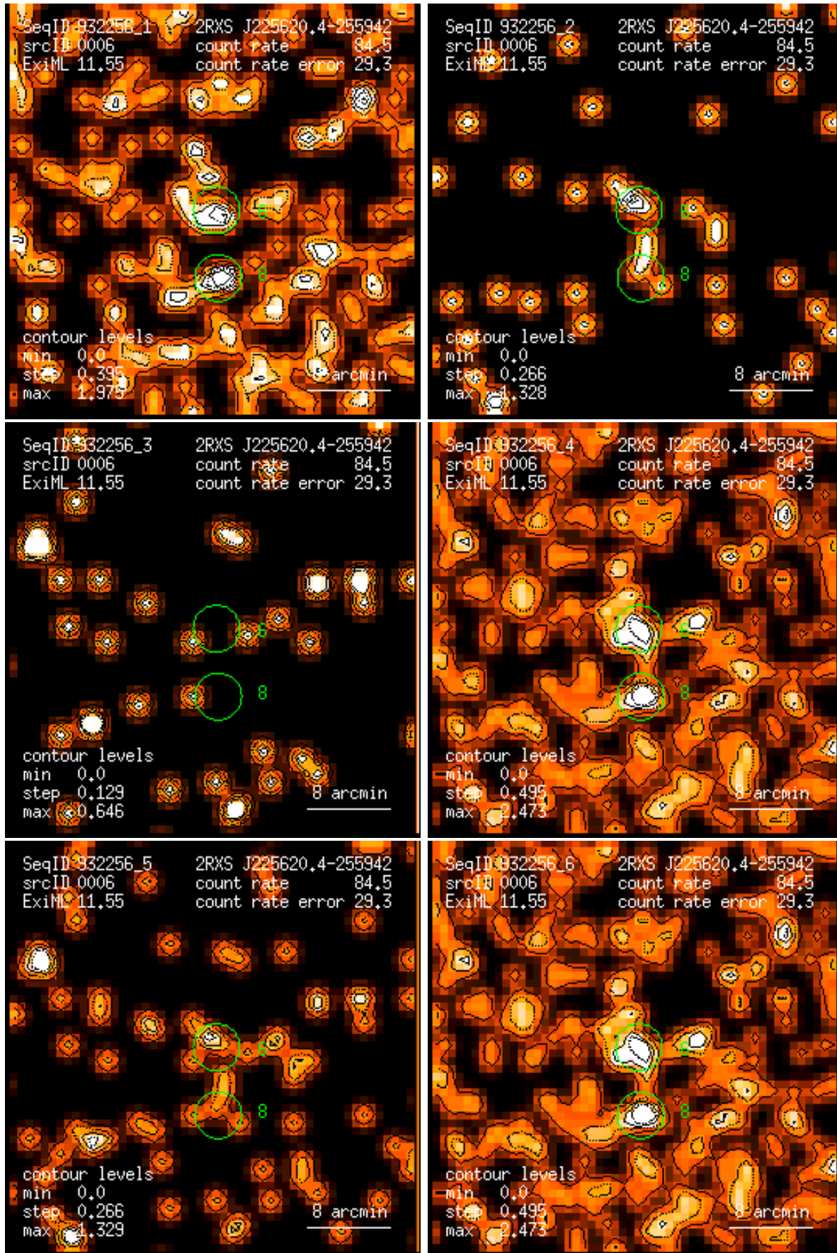
Figure 6: RASS 932256: detection 0006: band rate images, Gaussian filter: (1) PSPC channels 11 – 41, (2) 52 – 90, (3) 91 – 201, (4) 11 – 235, (5) 52 – 201, (6) 11 – 201. Broad band rates in counts/ks. Band rate contour levels in counts/ks/arcmin 2 .
