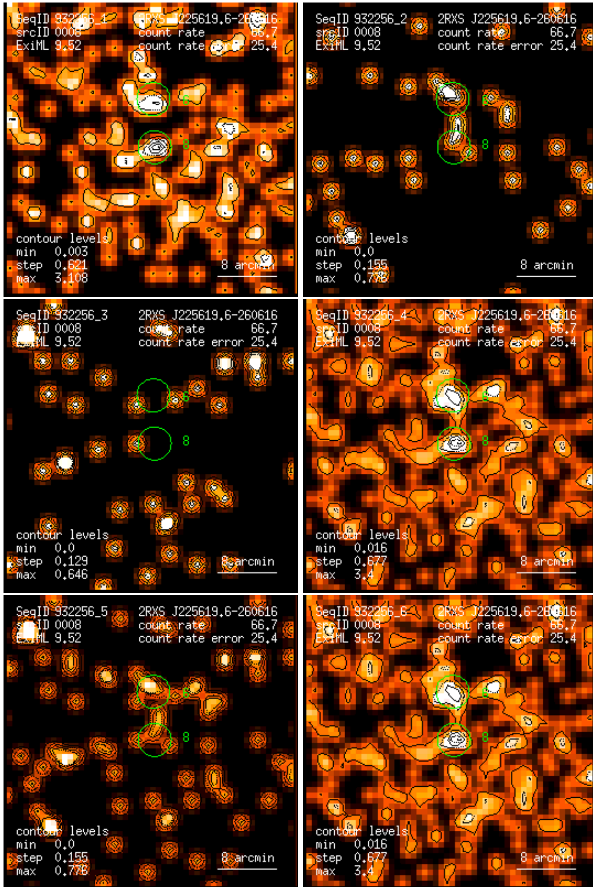
Figure 8: RASS 932256: detection 0008: band rate images, Gaussian filter: (1) PSPC channels 11 – 41, (2) 52 – 90, (3) 91 – 201, (4) 11 – 235, (5) 52 – 201, (6) 11 – 201. Broad band rates in counts/ks. Band rate contour levels in counts/ks/arcmin 2 .
