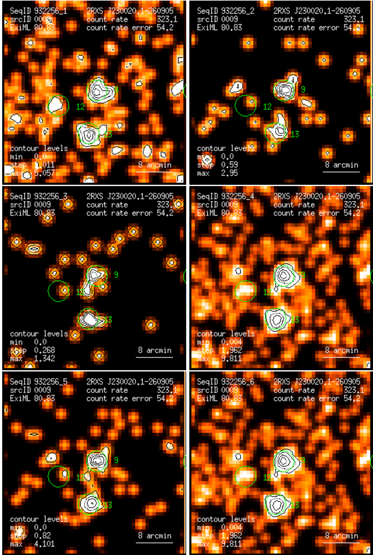
Figure 9: RASS 932256: detection 0009: band rate images, Gaussian filter: (1) PSPC channels 11 – 41, (2) 52 – 90, (3) 91 – 201, (4) 11 – 235, (5) 52 – 201, (6) 11 – 201. Broad band rates in counts/ks. Band rate contour levels in counts/ks/arcmin 2 .
