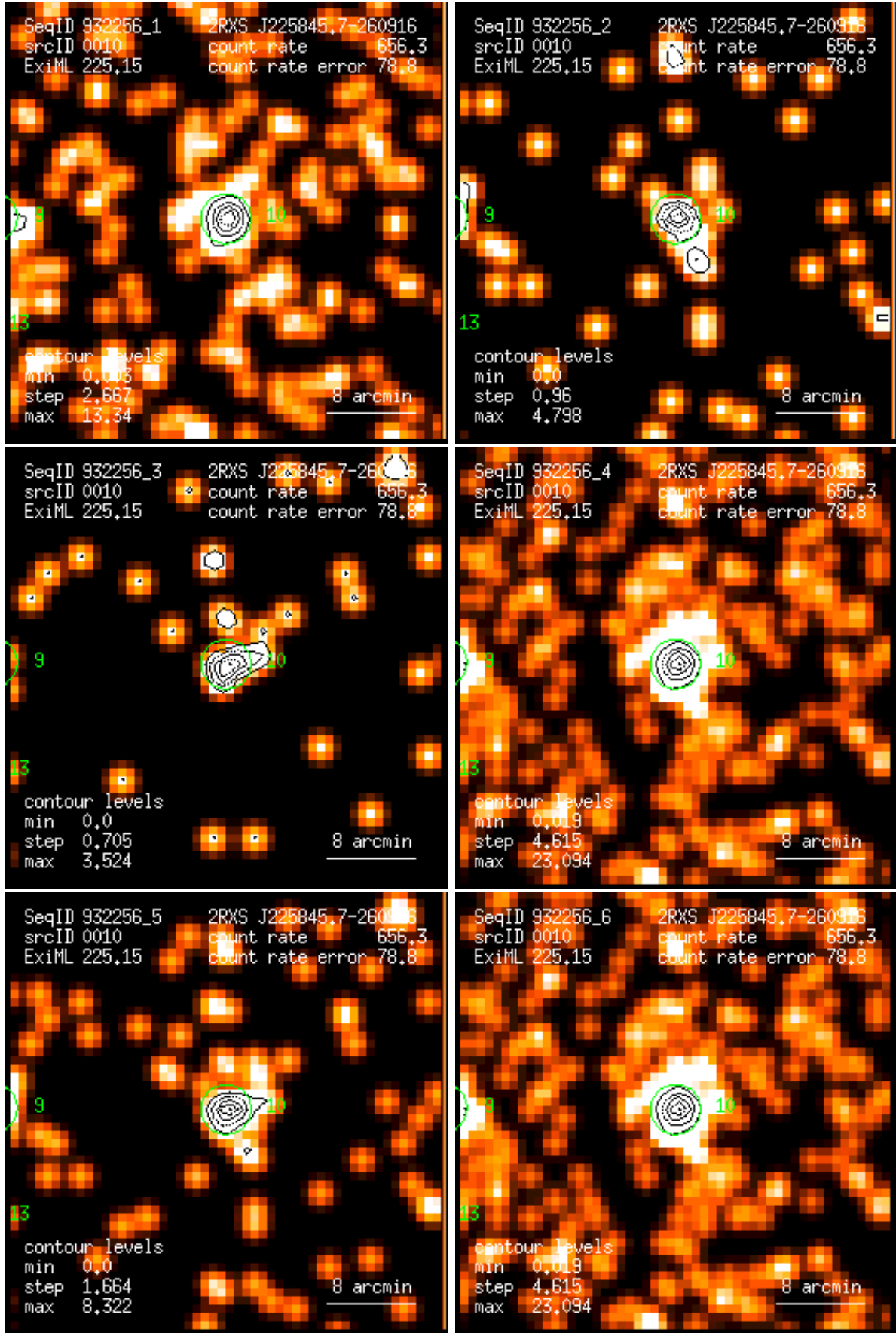
Figure 10: RASS 932256: detection 0010: band rate images, Gaussian filter: (1) PSPC channels 11 – 41, (2) 52 – 90, (3) 91 – 201, (4) 11 – 235, (5) 52 – 201, (6) 11 – 201. Broad band rates in counts/ks. Band rate contour levels in counts/ks/arcmin 2 .
