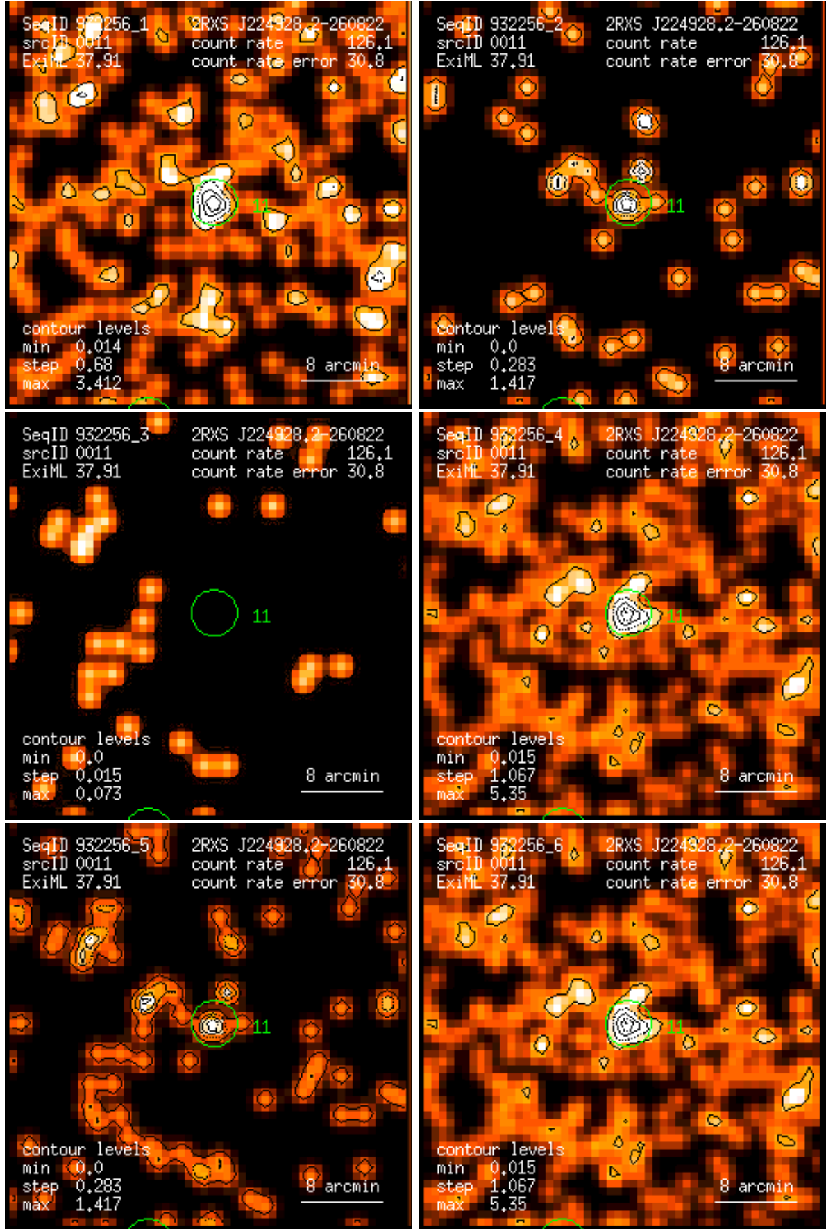
Figure 11: RASS 932256: detection 0011: band rate images, Gaussian filter: (1) PSPC channels 11 – 41, (2) 52 – 90, (3) 91 – 201, (4) 11 – 235, (5) 52 – 201, (6) 11 – 201. Broad band rates in counts/ks. Band rate contour levels in counts/ks/arcmin 2 .
