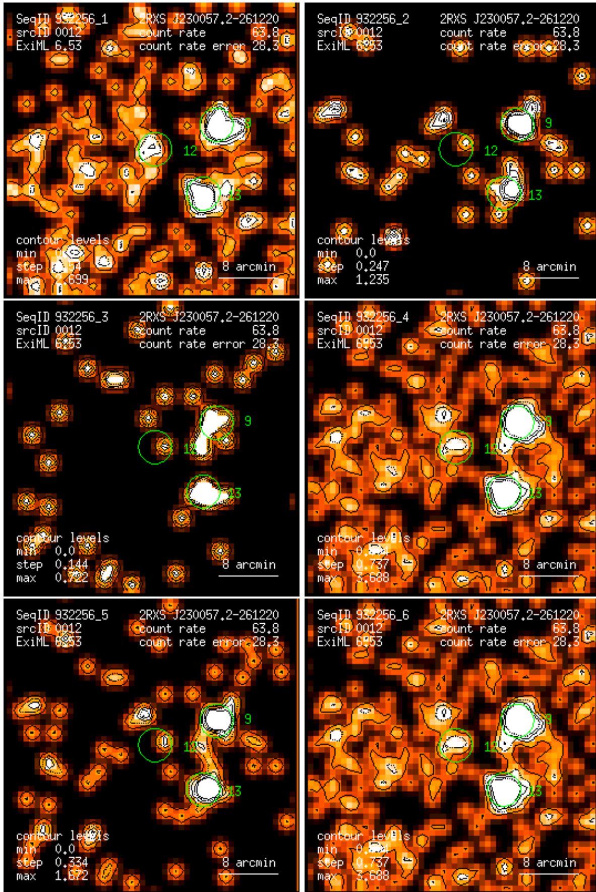
Figure 12: RASS 932256: detection 0012: band rate images, Gaussian filter: (1) PSPC channels 11 – 41, (2) 52 – 90, (3) 91 – 201, (4) 11 – 235, (5) 52 – 201, (6) 11 – 201. Broad band rates in counts/ks. Band rate contour levels in counts/ks/arcmin 2 .
