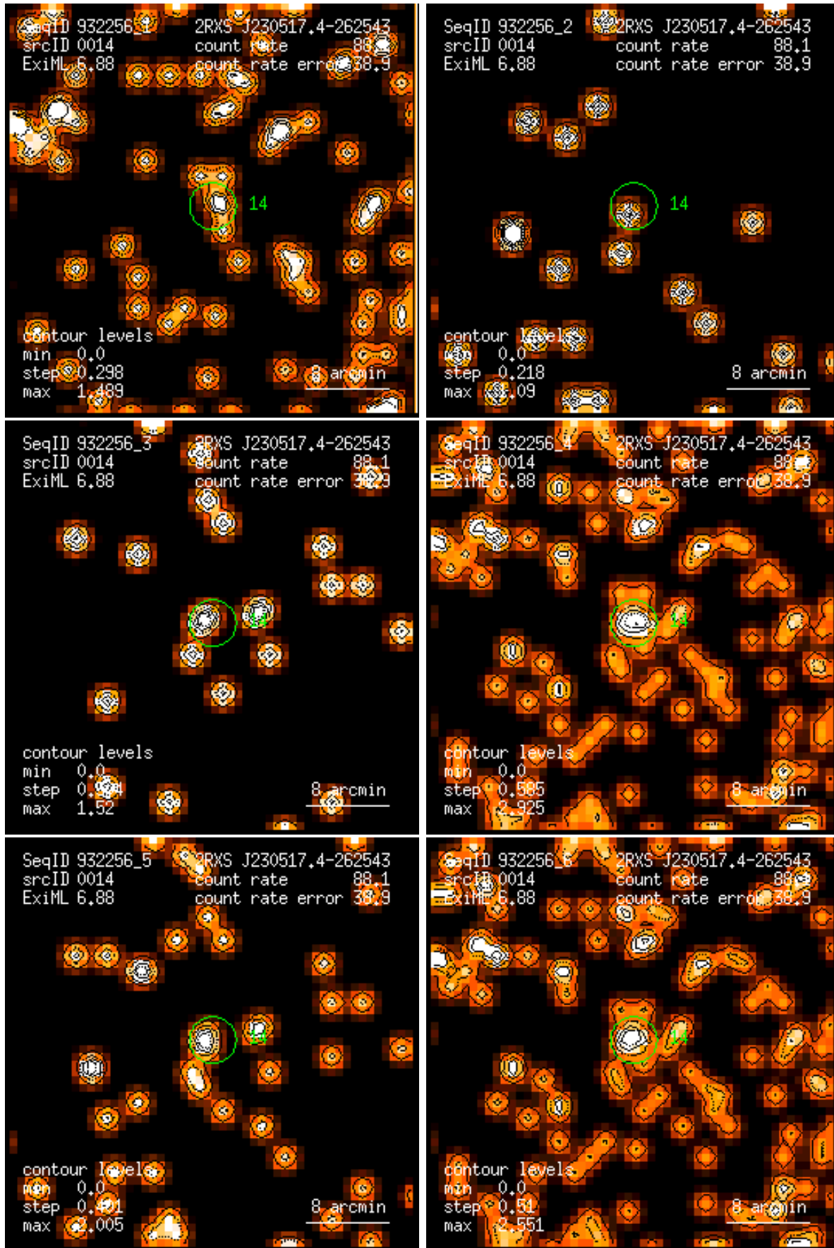
Figure 14: RASS 932256: detection 0014: band rate images, Gaussian filter: (1) PSPC channels 11 – 41, (2) 52 – 90, (3) 91 – 201, (4) 11 – 235, (5) 52 – 201, (6) 11 – 201. Broad band rates in counts/ks. Band rate contour levels in counts/ks/arcmin 2 .
