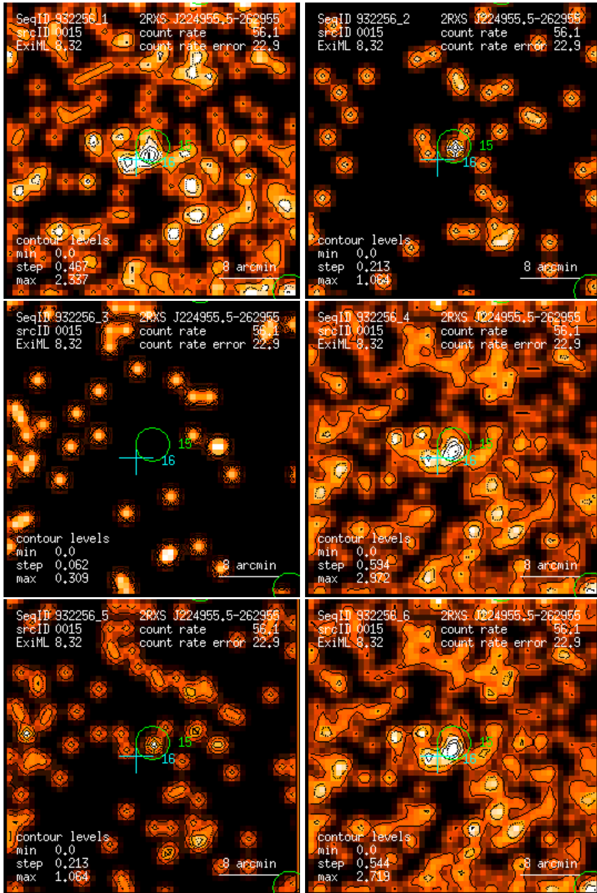
Figure 15: RASS 932256: detection 0015: band rate images, Gaussian filter: (1) PSPC channels 11 – 41, (2) 52 – 90, (3) 91 – 201, (4) 11 – 235, (5) 52 – 201, (6) 11 – 201. Broad band rates in counts/ks. Band rate contour levels in counts/ks/arcmin 2 .
