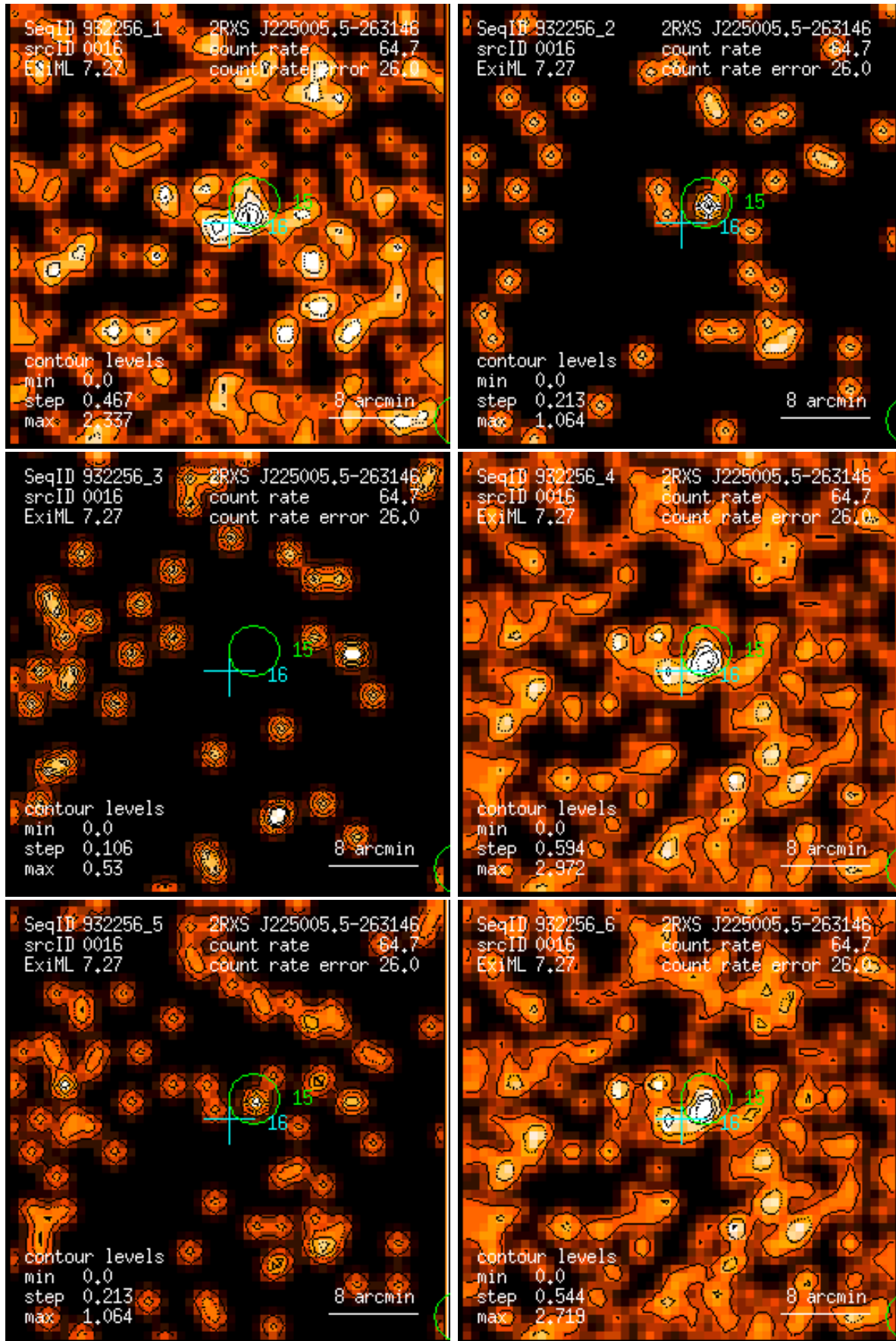
Figure 16: RASS 932256: detection 0016: band rate images, Gaussian filter: (1) PSPC channels 11 – 41, (2) 52 – 90, (3) 91 – 201, (4) 11 – 235, (5) 52 – 201, (6) 11 – 201. Broad band rates in counts/ks. Band rate contour levels in counts/ks/arcmin 2 .
