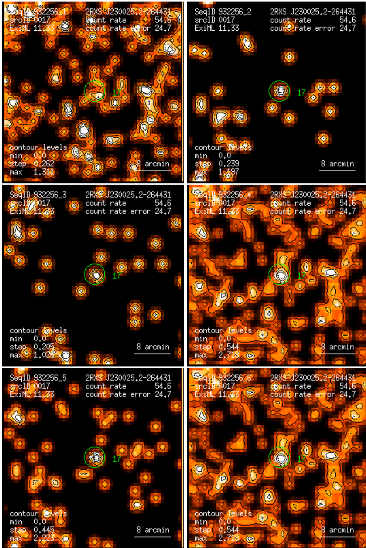
Figure 17: RASS 932256: detection 0017: band rate images, Gaussian filter: (1) PSPC channels 11 – 41, (2) 52 – 90, (3) 91 – 201, (4) 11 – 235, (5) 52 – 201, (6) 11 – 201. Broad band rates in counts/ks. Band rate contour levels in counts/ks/arcmin 2 .
