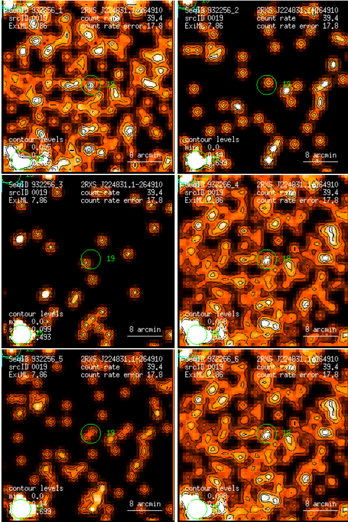
Figure 19: RASS 932256: detection 0019: band rate images, Gaussian filter: (1) PSPC channels 11 – 41, (2) 52 – 90, (3) 91 – 201, (4) 11 – 235, (5) 52 – 201, (6) 11 – 201. Broad band rates in counts/ks. Band rate contour levels in counts/ks/arcmin 2 .
