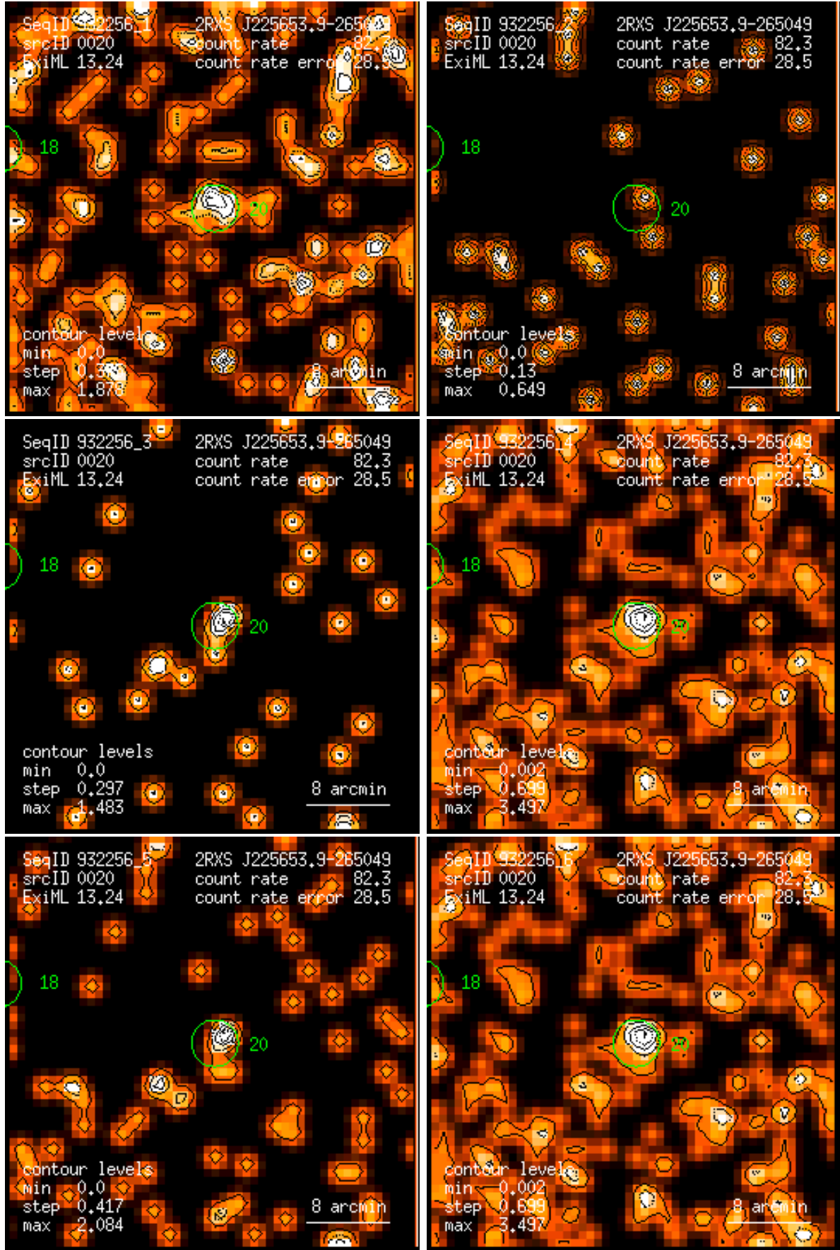
Figure 20: RASS 932256: detection 0020: band rate images, Gaussian filter: (1) PSPC channels 11 – 41, (2) 52 – 90, (3) 91 – 201, (4) 11 – 235, (5) 52 – 201, (6) 11 – 201. Broad band rates in counts/ks. Band rate contour levels in counts/ks/arcmin 2 .
