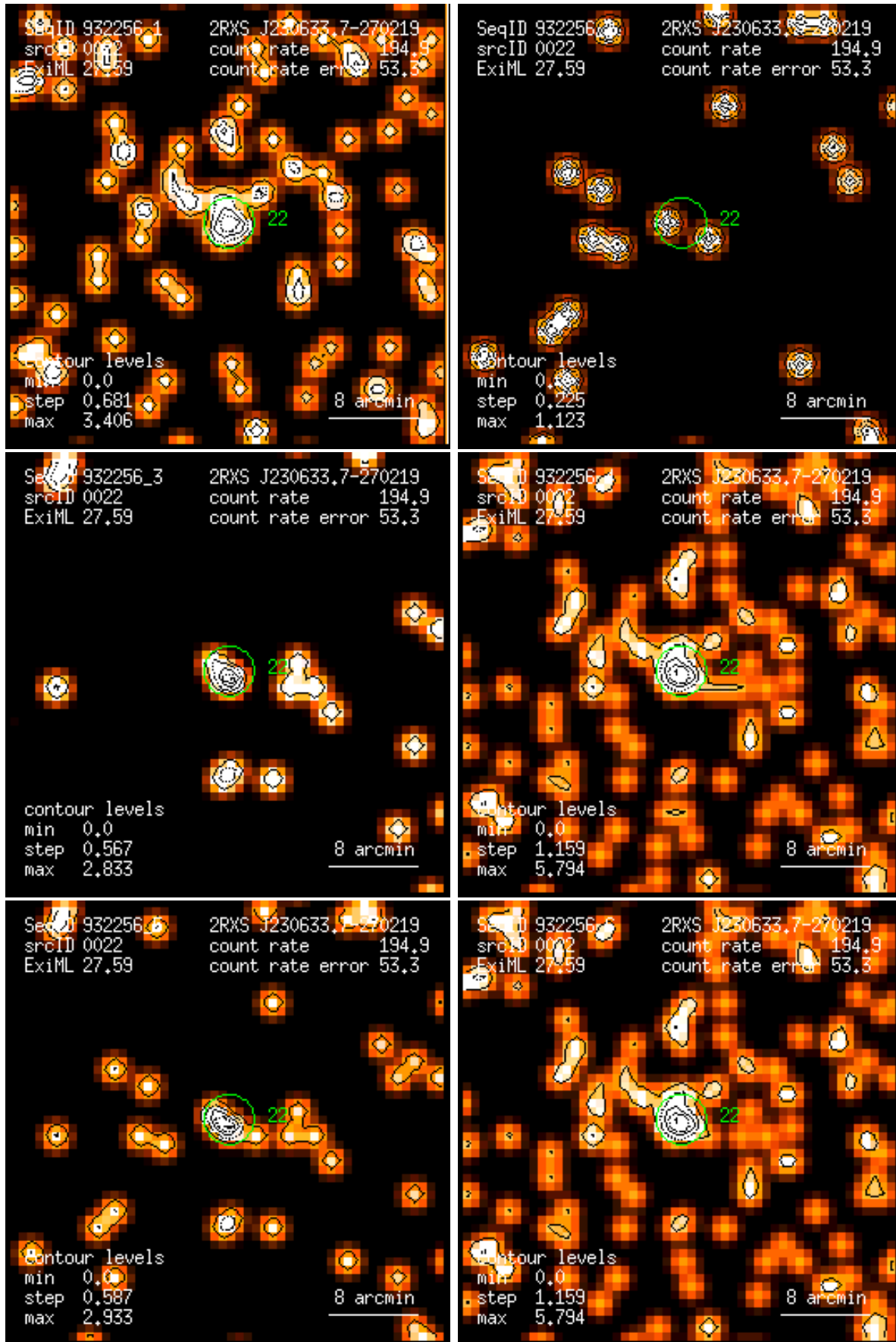
Figure 22: RASS 932256: detection 0022: band rate images, Gaussian filter: (1) PSPC channels 11 – 41, (2) 52 – 90, (3) 91 – 201, (4) 11 – 235, (5) 52 – 201, (6) 11 – 201. Broad band rates in counts/ks. Band rate contour levels in counts/ks/arcmin 2 .
