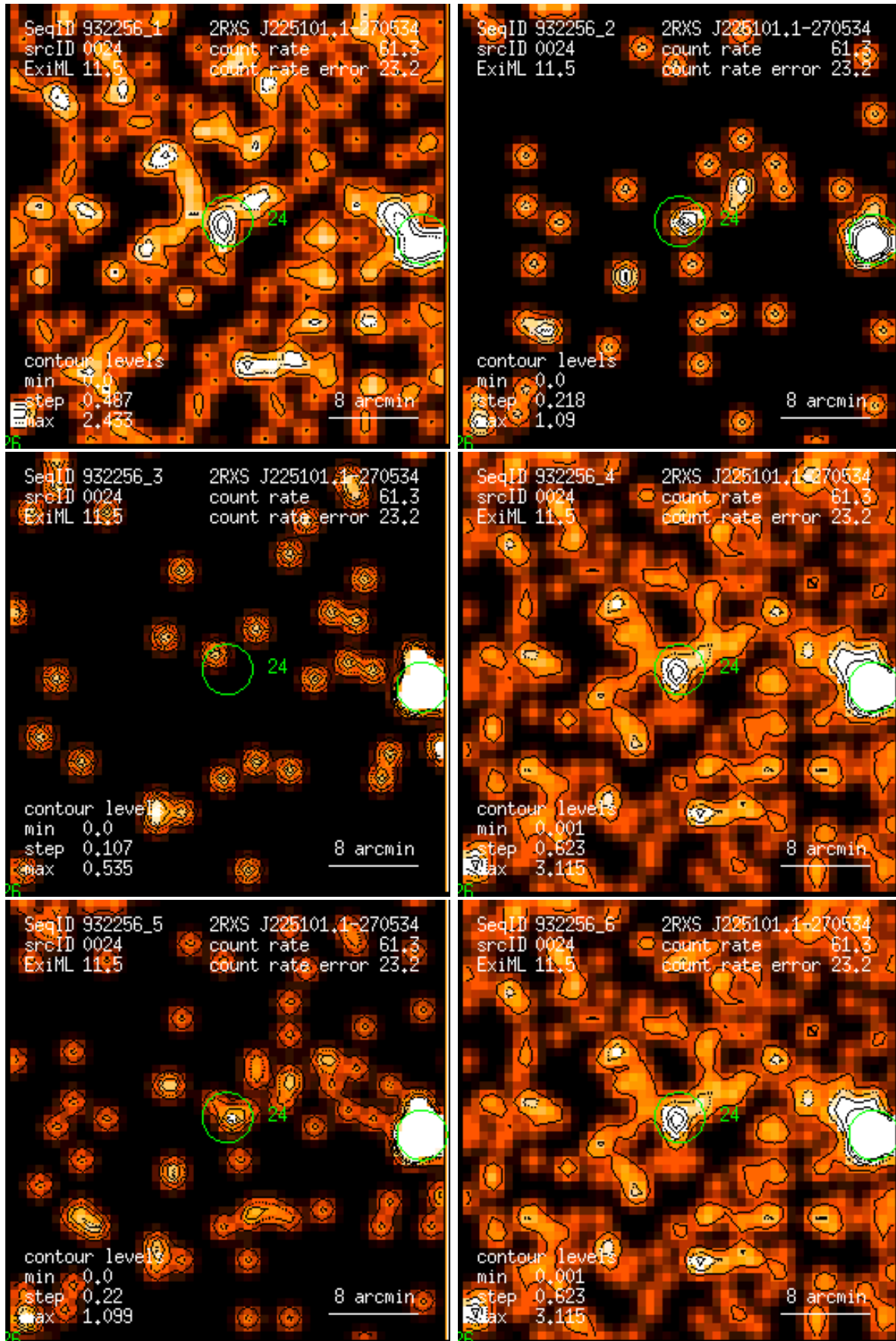
Figure 24: RASS 932256: detection 0024: band rate images, Gaussian filter: (1) PSPC channels 11 – 41, (2) 52 – 90, (3) 91 – 201, (4) 11 – 235, (5) 52 – 201, (6) 11 – 201. Broad band rates in counts/ks. Band rate contour levels in counts/ks/arcmin 2 .
