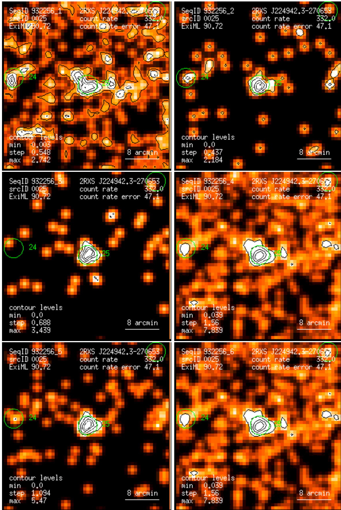
Figure 25: RASS 932256: detection 0025: band rate images, Gaussian filter: (1) PSPC channels 11 – 41, (2) 52 – 90, (3) 91 – 201, (4) 11 – 235, (5) 52 – 201, (6) 11 – 201. Broad band rates in counts/ks. Band rate contour levels in counts/ks/arcmin 2 .
