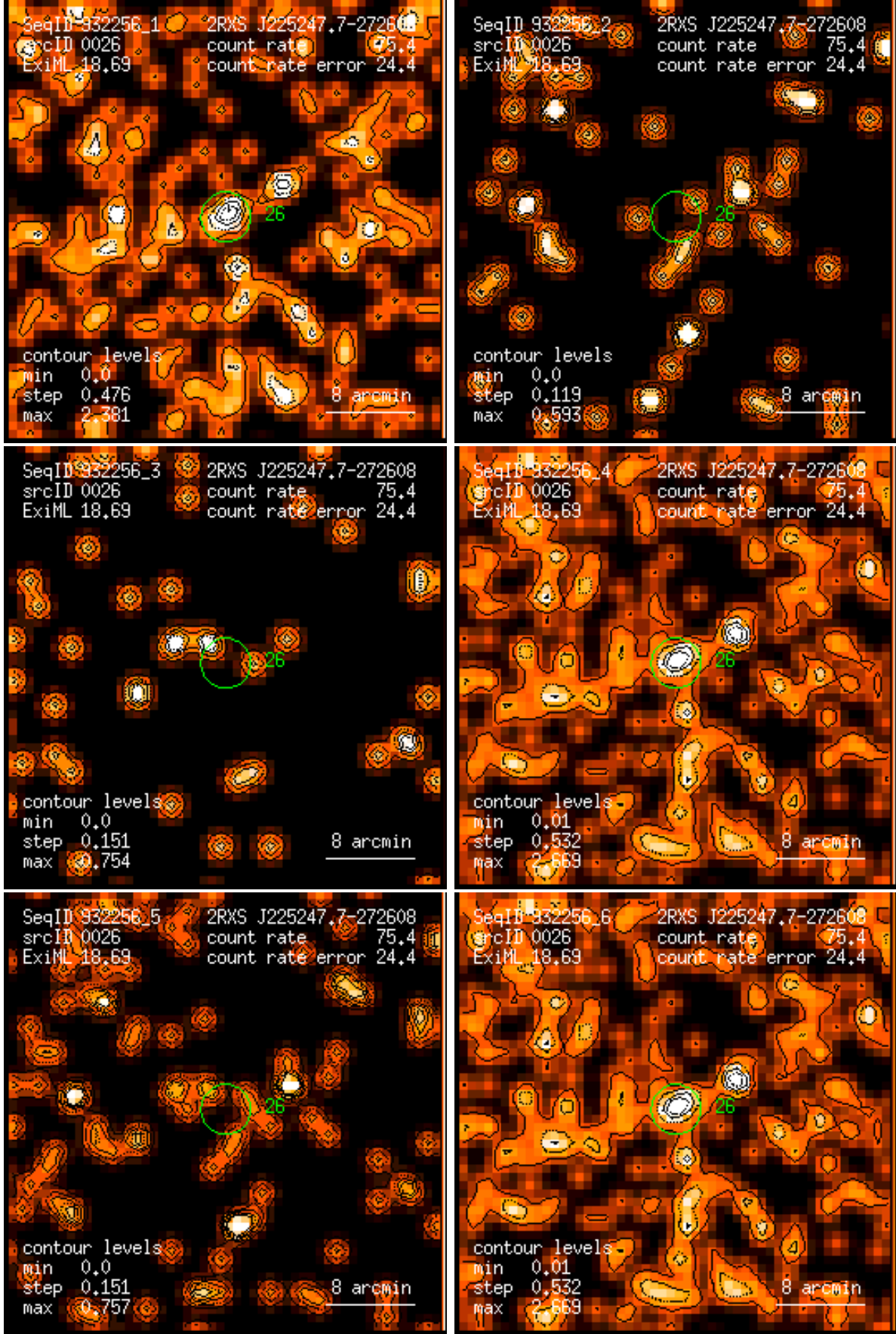
Figure 26: RASS 932256: detection 0026: band rate images, Gaussian filter: (1) PSPC channels 11 – 41, (2) 52 – 90, (3) 91 – 201, (4) 11 – 235, (5) 52 – 201, (6) 11 – 201. Broad band rates in counts/ks. Band rate contour levels in counts/ks/arcmin 2 .
