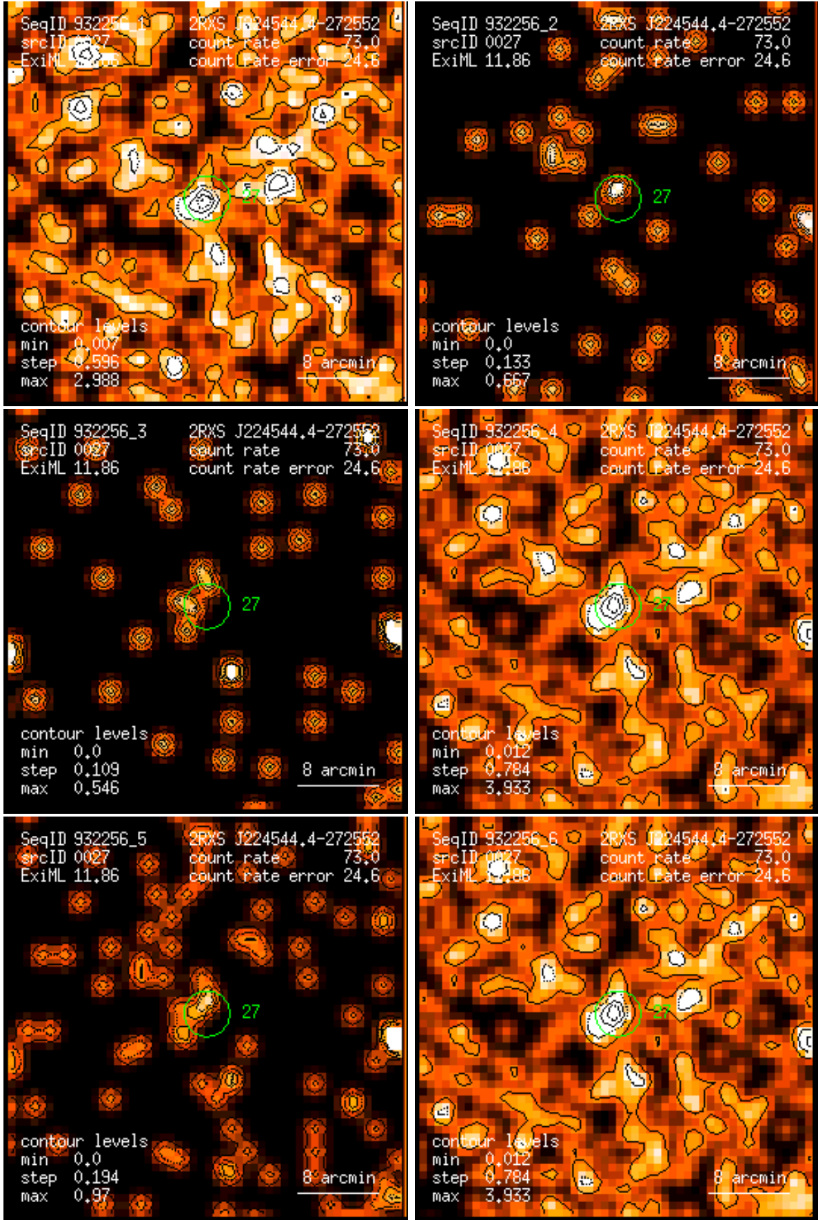
Figure 27: RASS 932256: detection 0027: band rate images, Gaussian filter: (1) PSPC channels 11 – 41, (2) 52 – 90, (3) 91 – 201, (4) 11 – 235, (5) 52 – 201, (6) 11 – 201. Broad band rates in counts/ks. Band rate contour levels in counts/ks/arcmin 2 .
