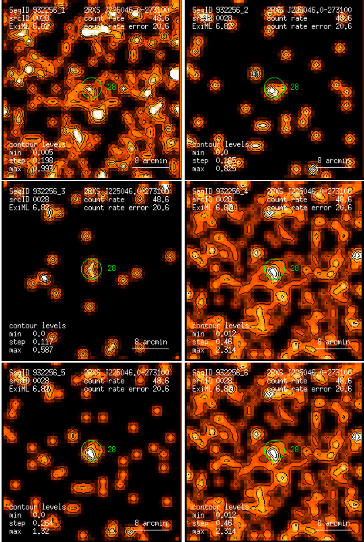
Figure 28: RASS 932256: detection 0028: band rate images, Gaussian filter: (1) PSPC channels 11 – 41, (2) 52 – 90, (3) 91 – 201, (4) 11 – 235, (5) 52 – 201, (6) 11 – 201. Broad band rates in counts/ks. Band rate contour levels in counts/ks/arcmin 2 .
