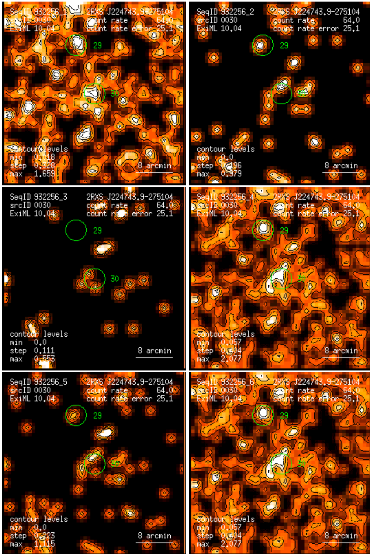
Figure 30: RASS 932256: detection 0030: band rate images, Gaussian filter: (1) PSPC channels 11 – 41, (2) 52 – 90, (3) 91 – 201, (4) 11 – 235, (5) 52 – 201, (6) 11 – 201. Broad band rates in counts/ks. Band rate contour levels in counts/ks/arcmin 2 .
